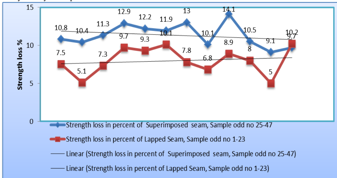
Figure 6: Comparison of Seam strength loss in percent between Lapped & Superimposed Seam.
