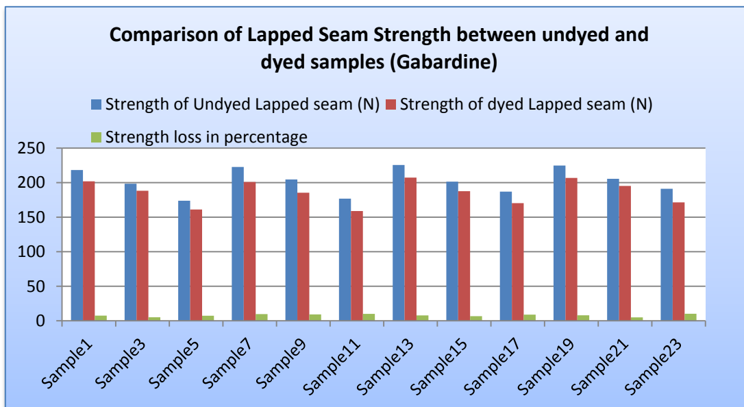
Figure 4: Comparison of Lapped Seam Strength in Newton (N) between un-dyed and dyed samples.
