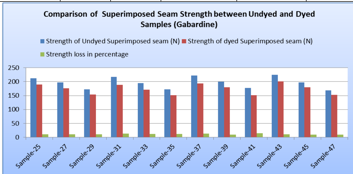
Figure 5: Comparison of Superimposed Seam Strength in Newton (N) between un-dyed and dyed Samples.
