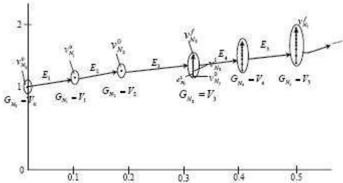
Figure 3: Multi-compound digraph
