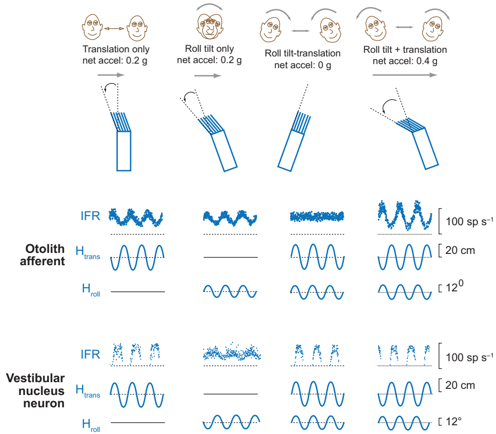
Figure 2 Instantaneous firing rate (IFR) from a primary otolith afferent ( top ) that encodes net linear acceleration, and a central vestibular nuclei neuron ( bottom ) that encodes translational motion during four movement protocols: Translation only, Tilt only, Tilt – Translation and Tilt + Translation (0.5 Hz). The stimulus ( bottom ) traces show sled position ( H_{trans} ) and roll tilt position ( H_{roll} ). Replotted with permission from Angelaki et al. (2004).
