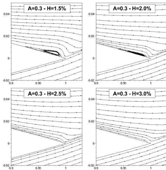
Fig. 29. Effect of suction jet width on eddies behind the airfoil at 16^\circ angle of attack.
