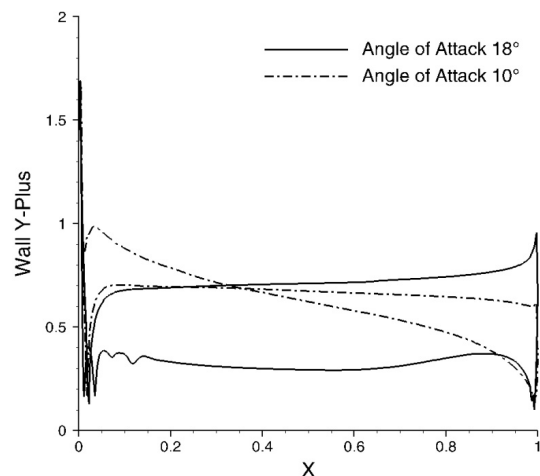
Fig. 3. Wall y-plus distribution over the NACA 0012 airfoil at angles of attack of 10^\circ and 18^\circ .
