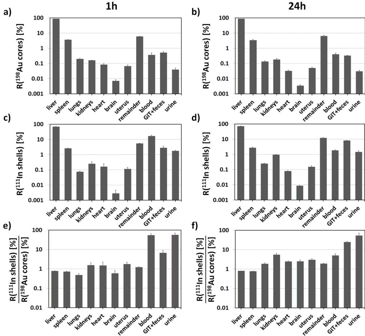
Figure 2: Biodistribution of double-labelled NPs. Au NPs (with core diameter d_c = 4.8 \pm 0.9 nm) with an ^{198}\text{Au} core radiolabel and an ^{111}\text{In} shell radiolabel had been intravenously injected into the tail vein of Wistar-Kyoto rats and their radioactivities were determined in different organs. Graphs show the quantitative balance (i.e. the sum of all ^{198}\text{Au} or ^{111}\text{In} radioactivities over all organs and tissues, the remaining carcass, and total faecal and urinary excretion is 100 %) of the 1 h and 24 h biodistribution of double-labelled Au NPs. The retentions R , given as mean data ( \pm SEM) are denoted in percent of the total radioactivity for the respective radio-isotope ( n = 4 animals per data point). “Remainder” represents radiolabels found in the remaining rest of the carcass after sampling of organs, i.e. soft tissues, skin and skeleton, etc. “GIT+feces” represents the radiolabels found in the gastro-intestinal-tract and in feces (note that after 1 hour no radiolabels were found in feces). “Blood” represents the total content of radiolabels as calculated from the measured content in the blood sample and the estimate of the total blood volume, cf. Methods. a, b) biodistribution of the ^{198}\text{Au} NP core radiolabel. c, d) biodistribution of
