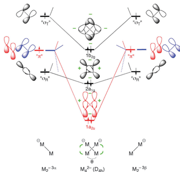
Fig. 8 Schematic molecular orbital interaction diagram of Al 4 2- constructed from two [M 2 ] 2- fragments at the BP86/TZ2P level (adapted from ref. 153). The positive and negative signs in green indicate whether there is a gain or loss of interaction when going from the D 4h to D 2h structure.
