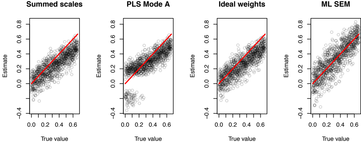
Figure 1 Comparison of regression with summed scales and PLS Mode A composites with latent variable SEM
