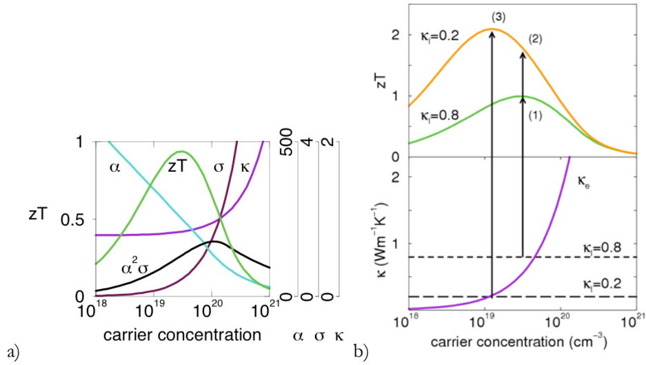
Figure 1. (a) Maximizing the efficiency ( zT ) of a thermoelectric involves a compromise of thermal conductivity ( \kappa , W/cmK) and Seebeck coefficient ( \alpha , \mu V/K) with electrical conductivity ( \sigma , 10^{-3} \Omega^{-1} cm ^{-1} ). Good thermoelectric materials typically are heavily doped semiconductors with a carrier concentration between 10^{19} and 10^{21} carriers/cm ^3 . Trends shown were modeled by \text{Bi}_2\text{Te}_3 , based on empirical data from Min and Rowe. 76 (b) Reducing the lattice thermal conductivity leads to a twofold benefit to the thermoelectric figure of merit. An optimized zT of 0.8 is shown (1) for a model system ( \text{Bi}_2\text{Te}_3 ) with a \kappa_l of 0.8 W/mK and a \kappa_e which is a function of the carrier concentration (purple). Reducing \kappa_l to 0.2 W/mK directly increases the zT to point (2). Additionally, lowering the thermal conductivity allows the carrier concentration to be reoptimized (reduced), leading to both a decrease in \kappa_e and a larger Seebeck coefficient. The reoptimized zT is shown at point (3).
