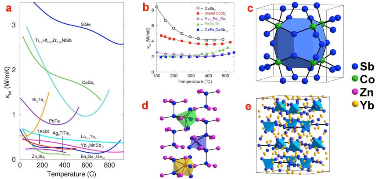
Figure 2. (a) Extremely low thermal conductivities are found in the recently identified complex material systems (such as \text{Yb}_{14}\text{MnSb}_{11} and \text{Zn}_4\text{Sb}_3 ) compared to most state-of-the-art thermoelectric materials ( \text{Bi}_2\text{Te}_3 , \text{PbTe} , \text{SiGe} ). (b) The high thermal conductivity of \text{CoSb}_3 is lowered when the electrical conductivity is optimized by doping (doped \text{CoSb}_3 ). The thermal conductivity is additionally lowered by alloying on the Co ( \text{Ru}_{0.5}\text{Pd}_{0.5}\text{Sb}_3 ) or Sb ( \text{FeSb}_2\text{Te} ) sites or by filling the void spaces ( \text{CeFe}_3\text{CoSb}_{12} ). 34 (c) The skutterudite structure is composed of tilted octahedral of \text{CoSb}_3 creating large void spaces shown in blue. (d) The room temperature structure of \text{Zn}_4\text{Sb}_3 has a crystalline Sb sublattice (blue) and highly disordered Zn sublattice containing a variety of interstitial sites (in polyhedra) along with the primary sites (purple). (e) The complexity of the \text{Yb}_{14}\text{MnSb}_{11} unit cell is illustrated, with [\text{Sb}_3]^{7-} trimers, [\text{MnSb}_4]^{9-} tetrahedra, and isolated Sb anions. The Zintl formalism describes these units as covalently bound with electrons donated from the ionic \text{Yb}^{2+} sublattice (yellow).
