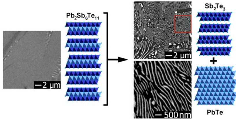
Figure 4. Truly nanostructured thermoelectrics may be formed by the solid state partitioning of a precursor phase. The metastable \text{Pb}_2\text{Sb}_6\text{Te}_{11} phase (left) will spontaneously assemble into lamellae of \text{Sb}_2\text{Te}_3 and \text{PbTe} . These domains are visible with backscattering SEM, with the dark regions corresponding to \text{Sb}_2\text{Te}_3 and the light regions to \text{PbTe} . Electron backscattering diffraction reveals that the lamellae are oriented with coherent interfaces, shown schematically (right).
