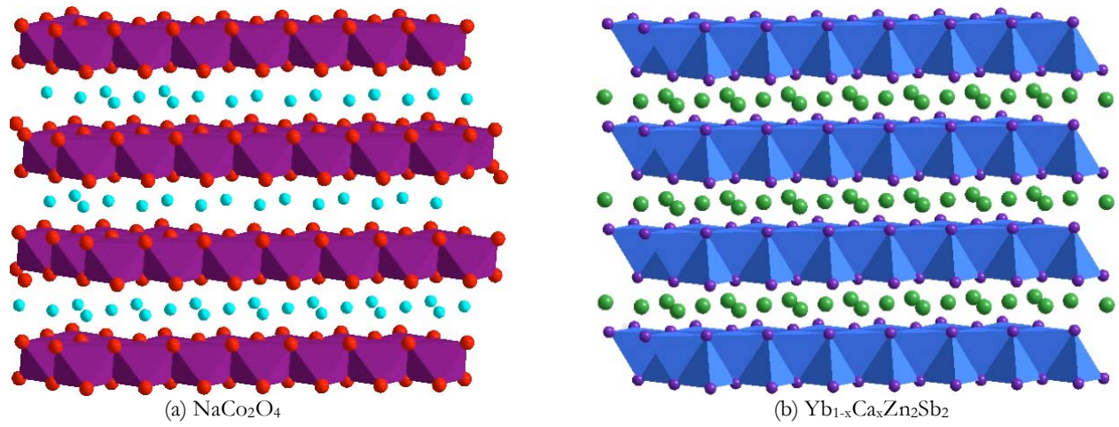
Figure 3. Substructure approach to separate the electron-crystal and phonon-glass attributes of a thermoelectric. Both the (a) \text{NaCo}_2\text{O}_4 and (b) \text{Yb}_{1-x}\text{Ca}_x\text{Zn}_2\text{Sb}_2 structures contain ordered layers (polyhedra) separated by disordered cation monolayers, creating electron-crystal phonon-glass structures.
