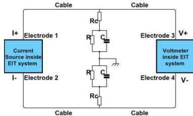
Figure 1: Circuit diagram for single channel calibration.
