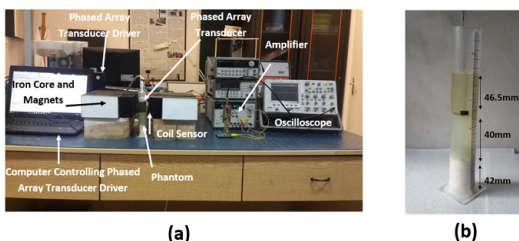
Figure 1: (a) Experimental setup for MAET method (b) Phantom.
