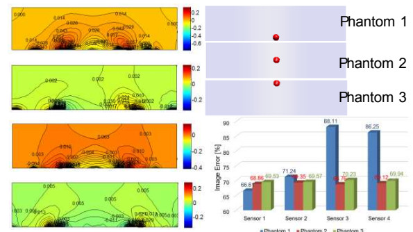
Figure 3: Sensitivity and image error analysis of each sensor. The left part is the vertical slice of sensitivity (from top to bottom: sensor 1 to sensor 4). Right top shows side views of three phantoms. Right bottom shows the image errors.
