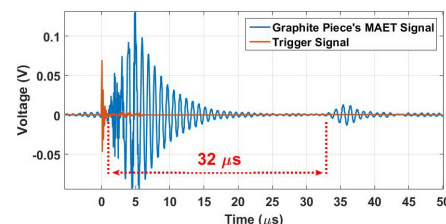
Figure 2: MAET signal from graphite-agar-gel interface at 32 \mu s .
