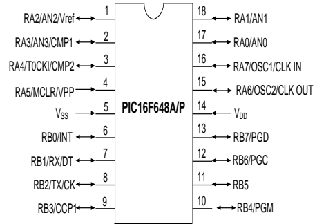
Figure 2.10: The pin out orientation of the PIC16F648A
