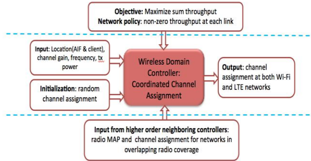
Figure 6. Channel allocation for wireless network using inter-network cooperation
