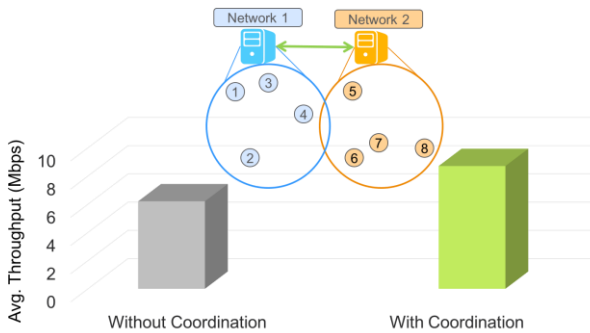
Figure 5. RadioMap Coordination Mechanisms Prototype Based Results.
