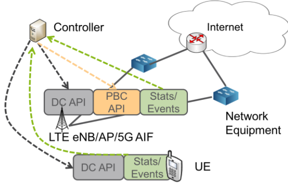
Figure 3. APIs for variety of air interfaces/common functions towards SDNization of wireless access networks.
