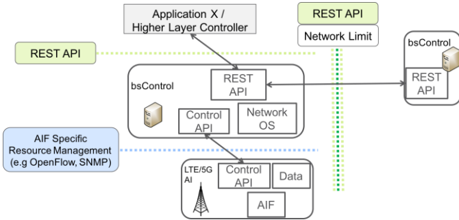
Figure 4. Prototype architecture diagram.
