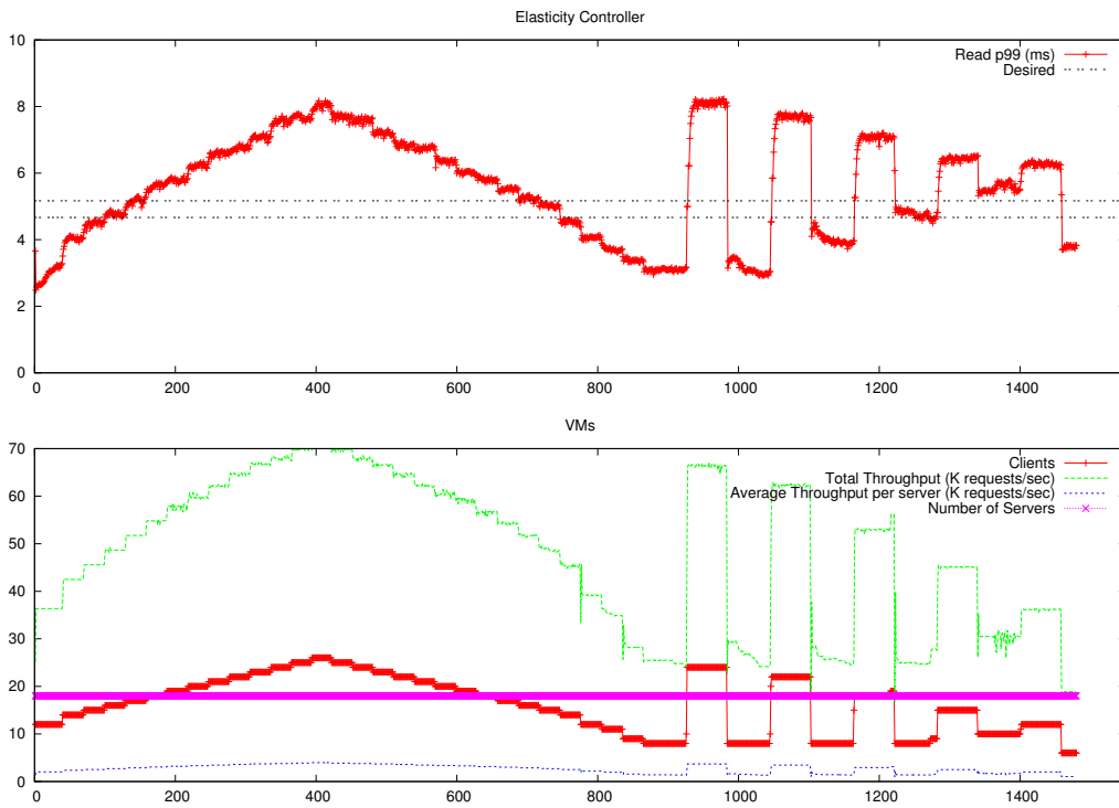
Figure 9: Performance of Voldemort without ElastMan with fixed number of servers (18 virtual servers) under gradual diurnal workload (0-900 min) and under workload with spikes (900-1500 min)
