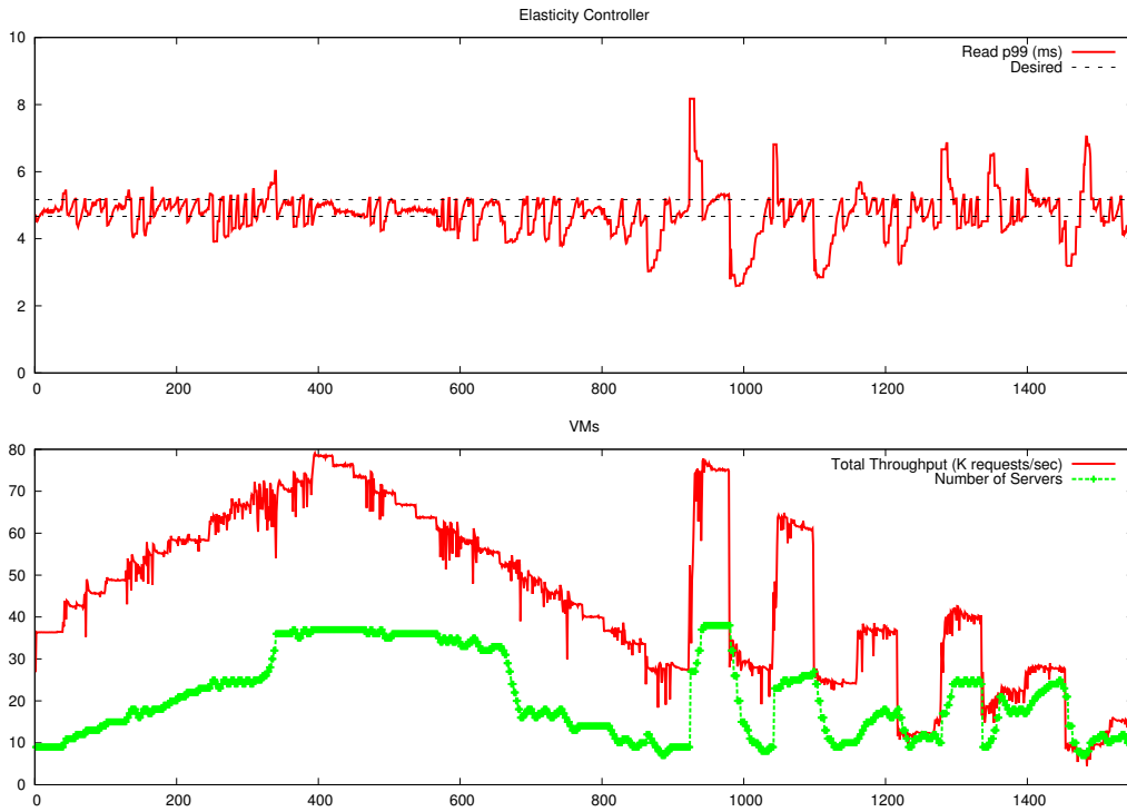
Figure 8: Performance of Voldemort with ElastMan under gradual diurnal workload (0-900 min) and under workload with spikes (900-1500 min)
