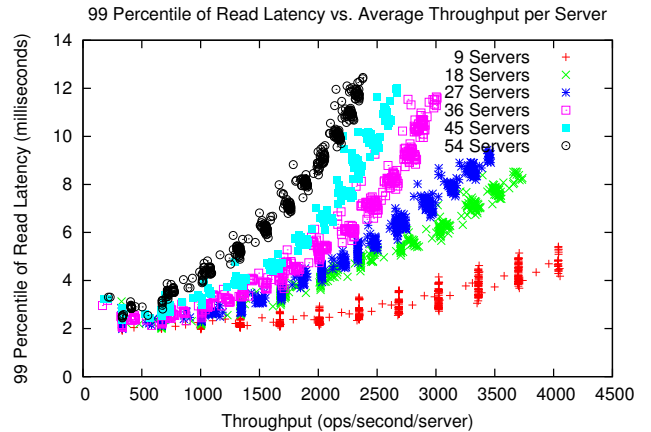
Figure 7: 99th percentile of read operations latency versus average throughput per server
