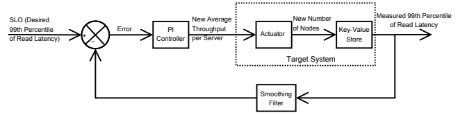
Figure 2: ElastMan Feedback Control
