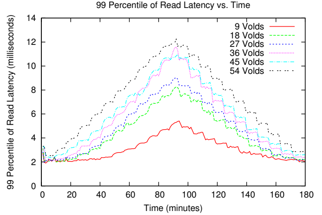
Figure 6: 99th percentile of read operations latency versus time under relatively similar workload
