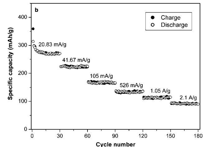
Fig. 5 Electrochemical characterization of the carbon-Fe-LiF nanocomposite. (a) Specific capacity as a function of cycle number. Inset: Galvanostatic charge/discharge time vs. voltage. (b) Specific capacity vs. cycle number at various current densities; the nanocomposite cycled between 4.3 and 0.5 V for 30 cycles at each current density.
