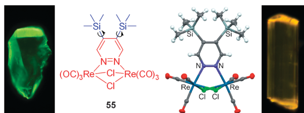
Fig. 22 Photographs of crystals of 55 taken under illumination of a UV lamp. Reproduced with permission from ref. 109. Copyright (2010) American Chemical Society.
