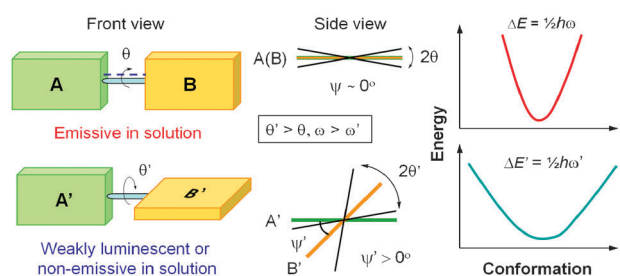
Fig. 17 Schematic illustration of the relationship among conformational planarity, torsional motion, energy surface, and luminescence efficiency. Symbols: \psi^{(l)} = dihedral angle between chromophoric units A (l) and B (l) , \theta^{(l)} = rotation amplitude, and \omega^{(l)} = frequency or wavenumber.
