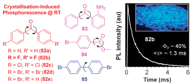
Fig. 45 Examples of room-temperature organic phosphorogens ( 82–85 ), whose emissions are induced by crystal formation. Phosphorescence decay curve of 4,4'-difluorobenzophenone ( 82b ) and photograph of its crystals taken under UV illumination. Reproduced with permission from ref. 158. Copyright (2010) American Chemical Society.
