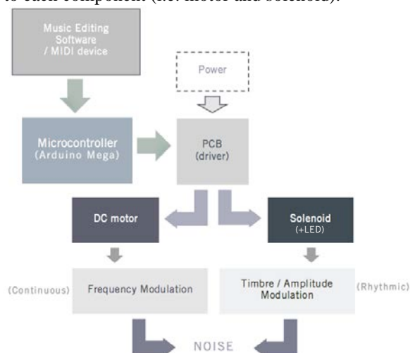
Figure 8 System overview
