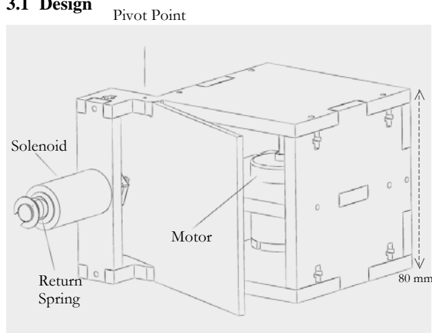
Figure 6 Mutor parts and design sketch
