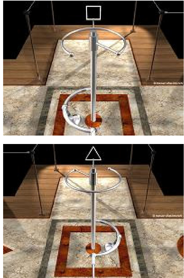
Figures 5/6. Transformation in 3D of square and triangle.
