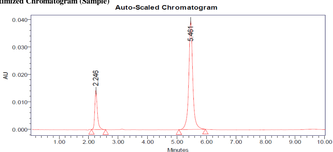
Figure-2: Optimized Chromatogram (Sample)
