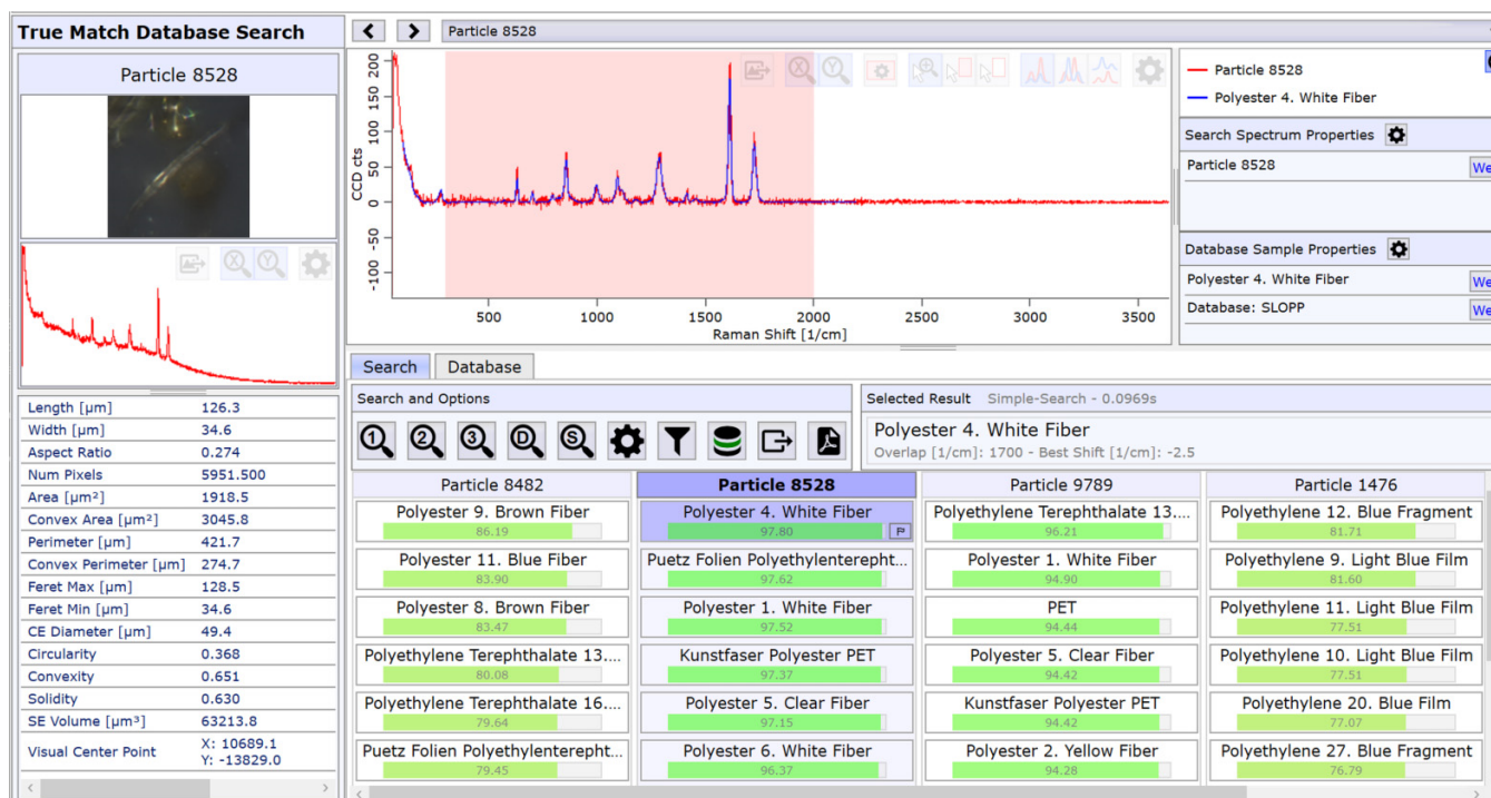
Fig. 2. Example of a microplastic particle identified by Raman spectroscopy using a combination of several spectral databases (Cabernard et al. 2018; Munno et al. 2020; von der Esch et al. 2020a). Left side: Particle image, raw Raman spectra, and particle details derived by image analysis. Right side: Processed spectra (red) and assigned library spectrum (blue) for the selected particle and reference spectra (highlighted in violet) combined with material name and further information.
