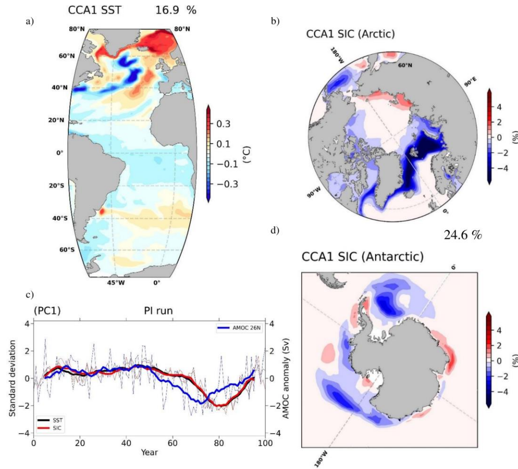
Figure 3 | The first simulated coupled Atlantic SST - Global SIC patterns identified through CCA between the corresponding AWIESM2.1 “Pre Industrial” annual anomalies extending over 100 years. Pattern of SST (°C) (a) and of the Arctic (b) and Antarctic (d) SIC (%) from the first coupled CCA pair. Their associated time series (c) with SIC (red line), SST (black line) are plotted with an 11yr running mean and have a correlation with the simulated AMOC Index, defined as the time series of annual-mean anomaly of the maximum volume transport streamfunction at 26.5°N (Sv) (blue line) of 0.37 (95% significance level).
