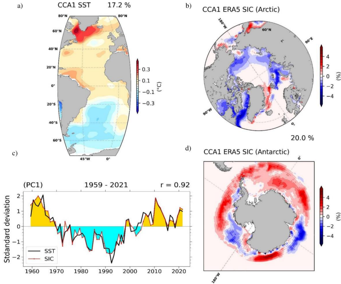
Figure 1 | The first coupled Atlantic Sea surface temperature (SST) - Global sea ice concentration (SIC) patterns identified through Canonical Correlation Analysis (CCA) between the corresponding ErSSTv5 and ERA5 Reanalysis annual detrended anomalies extending over the 1959 - 2021 period..
