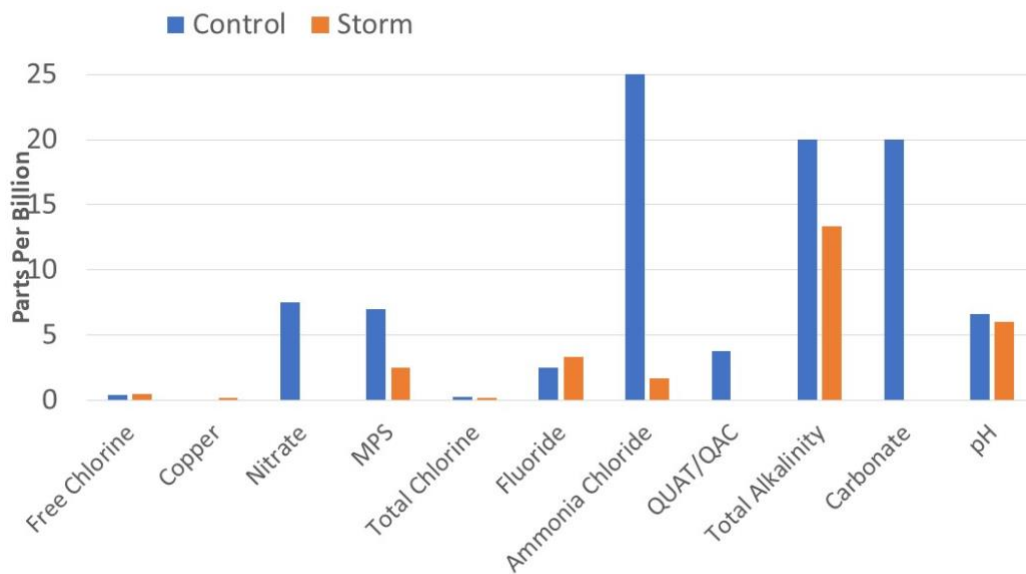
Fig. 5. illustrates the effects of storm events on the levels of chemicals present in the Schuylkill River. Overall, the relative concentrations of chemicals decreased with the influx of water from the storms, and the total hardness (representing all minerals, not shown) experienced a significant decrease. However, two days after the storm, levels of free chlorine, copper, and fluoride showed an increase. Additionally, the pH of the water decreased post-storm.
