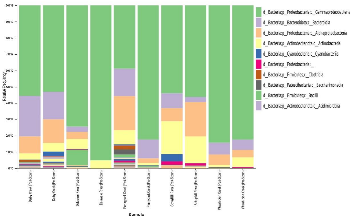
Fig. 8. Microbial Diversity of Philadelphia Surface Waters Pre and Post Storm Events.
