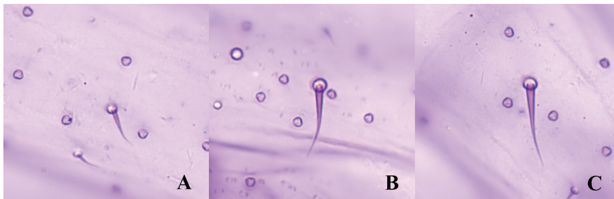
Figure 3. Dorsal setae on Planococcus camelliae Zhang, sp. nov.: A small seta B large seta with trilobular pore next to setal base C large seta without trilobular pore next to setal base.
