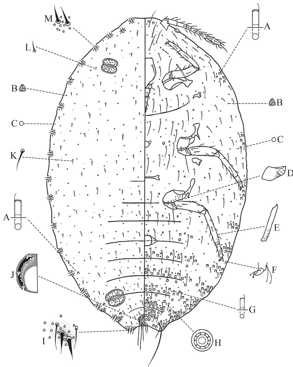
Figure 2. Adult female of Planococcus camelliae Zhang, sp. nov.: A Large oral collar tubular duct B trilocular pore C discoidal pore D hind coxa E hind tibia F claw G small oral collar tubular duct H multilocular disc pore I anal lobe cerarius ( C_{18} ) J anal ring K large dorsal seta L small dorsal seta M cerarius on head.
