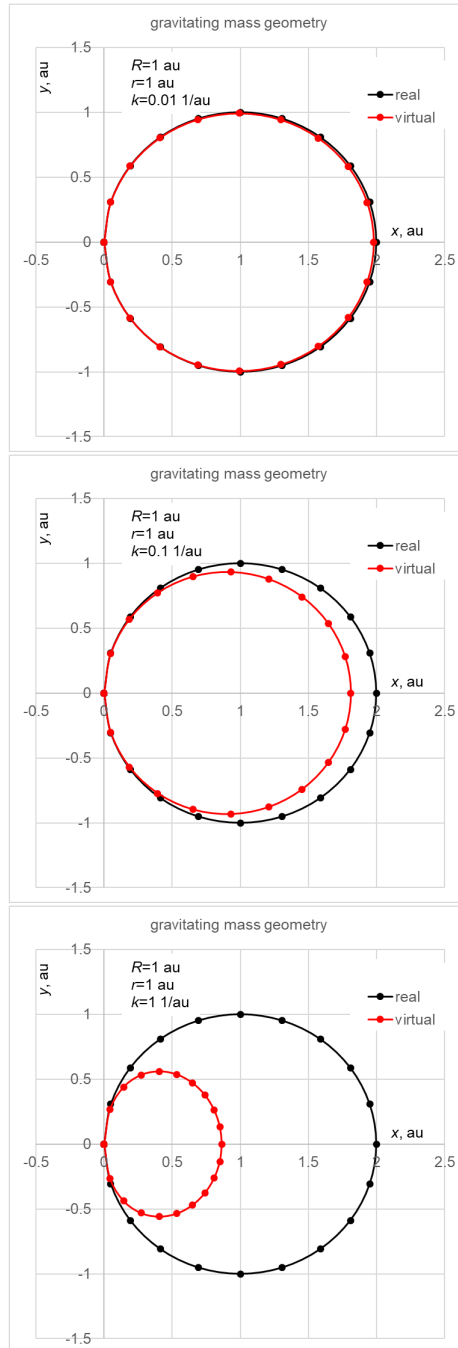
Figure 30: Real sphere in black, gravitoid (virtual) shape in red for three values of k and r = R = 1 .
