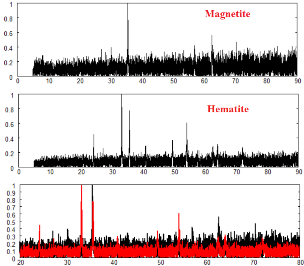
XRD data for Magnetite and Hematite (in the lower panel, in black data of magnetite and in red of hematite). Data from RRUFF, https://rruff.info/magnetite/display=default/R060191 and https://rruff.info/hematite/display=default/R040024 .
