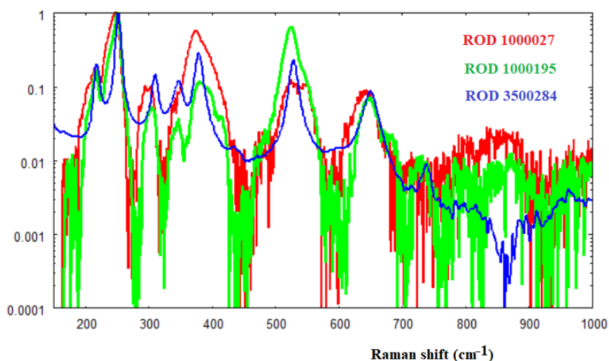
Fig.7b: The same as in Fig.7a with semi log scale.
