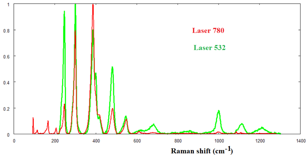
Fig. 9: Raman spectra of Goethite sample R120086.
