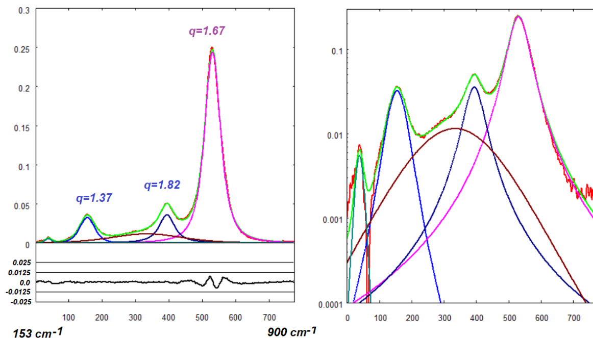
Fig.2: Deconvolution of a part of the Magnetite spectrum obtained by means of q -Gaussian functions. The best fit (green) is onto data (red) provided by Kumar et al., 2019; frequency range is from 153 to 900 \text{cm}^{-1} (see Fig.1). For the deconvolution, five q -Gaussians have been used. For the stronger peaks the values of the q -parameters are given in the figure. A quite flat q -Gaussian seems being related to a band at 475 \text{cm}^{-1} . In the following discussion of the magnetite Raman spectrum, we will see that a band at 470-472 \text{cm}^{-1} has been detected. In the lower part of the plot, the misfit is also proposed. On the right, the same fit is shown with the log scale for y-axis (semi log scale). Data and q -Gaussians are given as functions of integers n (equally spaced points used in fitting), for the x-axis which is representing the Raman shift. A convenient scale is used for the y-axis (intensity axis). The fitting calculation is obtained by minimizing the sum of the squares of the deviations.
