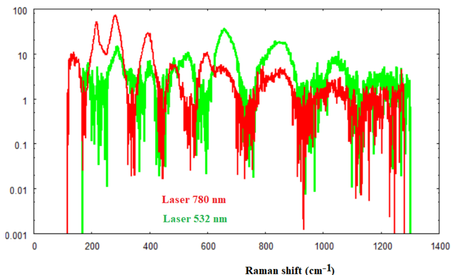
Fig.6b: The same as in Fig. 6a in semi logarithmic scale.
