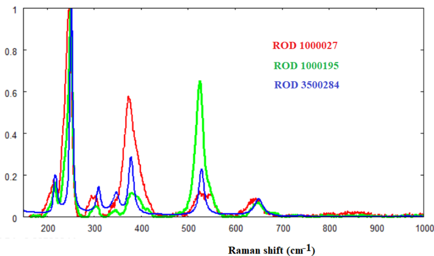
Fig.7a: Raman spectra of Lepidocrocite from Raman Open Database (ROD). ROD 1000027 (laser 780 nm) data courtesy Wyckoff, 1963, https://solsa.crystallography.net/rod/1000027.rod ; ROD 1000195 (laser 532) data courtesy Wyckoff, 1963, https://solsa.crystallography.net/rod/1000195.rod ; and ROD 3500284 (laser 633 nm) data courtesy Kumar et al., 2019, https://solsa.crystallography.net/rod/3500284.rod
