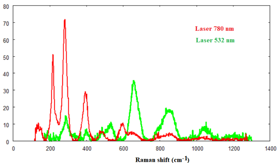
Fig.6a: Maghemite Raman spectra from RRUFF Project website.
