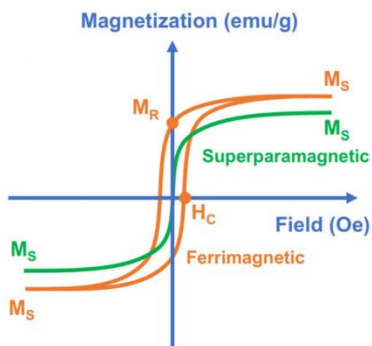
The image shows the magnetization versus the applied field ( M\text{--}H ) for superparamagnetic (SPM) (green color) and ferrimagnetic (FM) (orange) \text{Fe}_3\text{O}_4 nanoparticles. Image courtesy Nguyen et al., 2021, article distributed under https://creativecommons.org/licenses/by/4.0/
