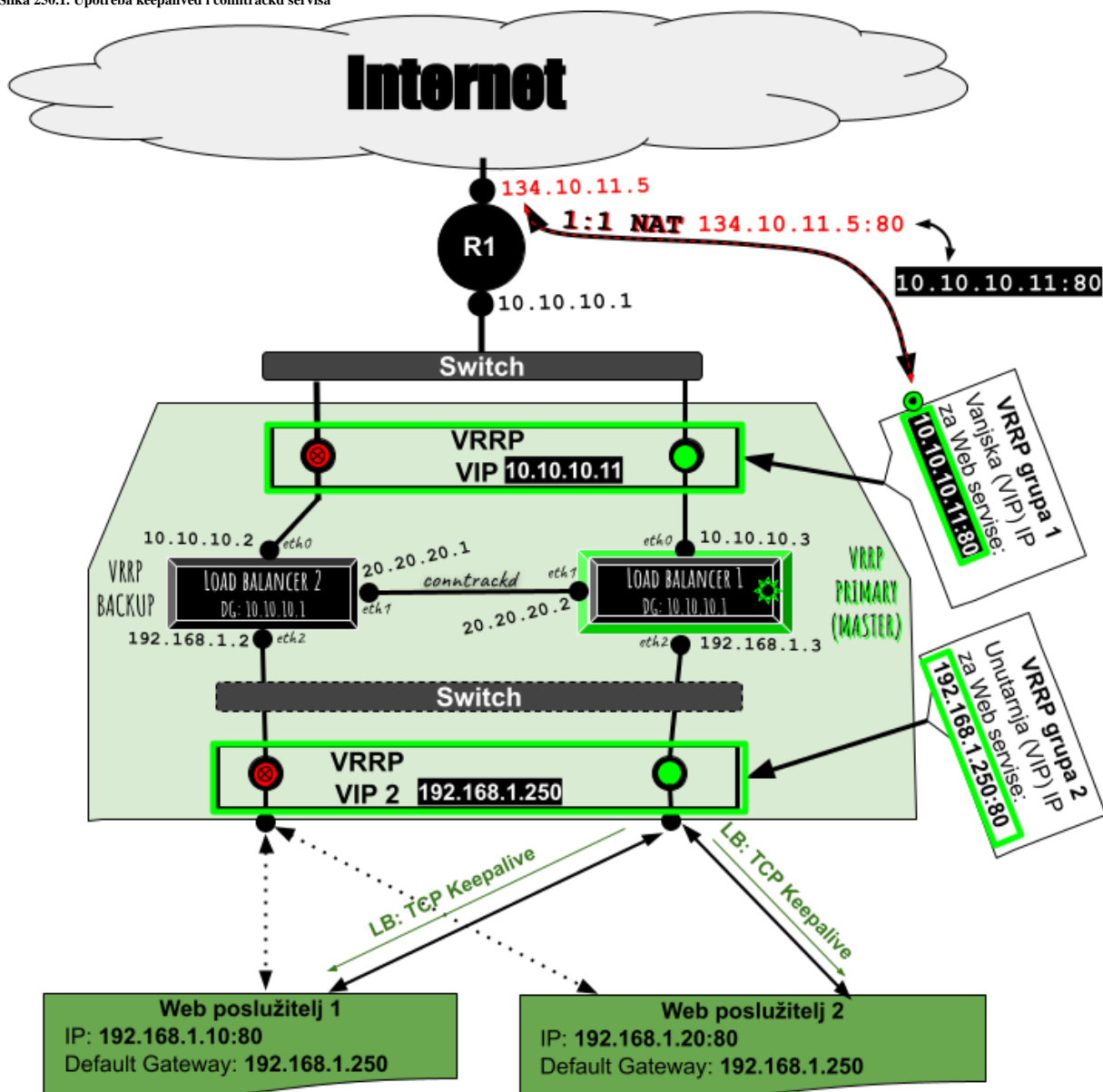
Slika 250.1. Upotreba keepalived i contrackd servisa
