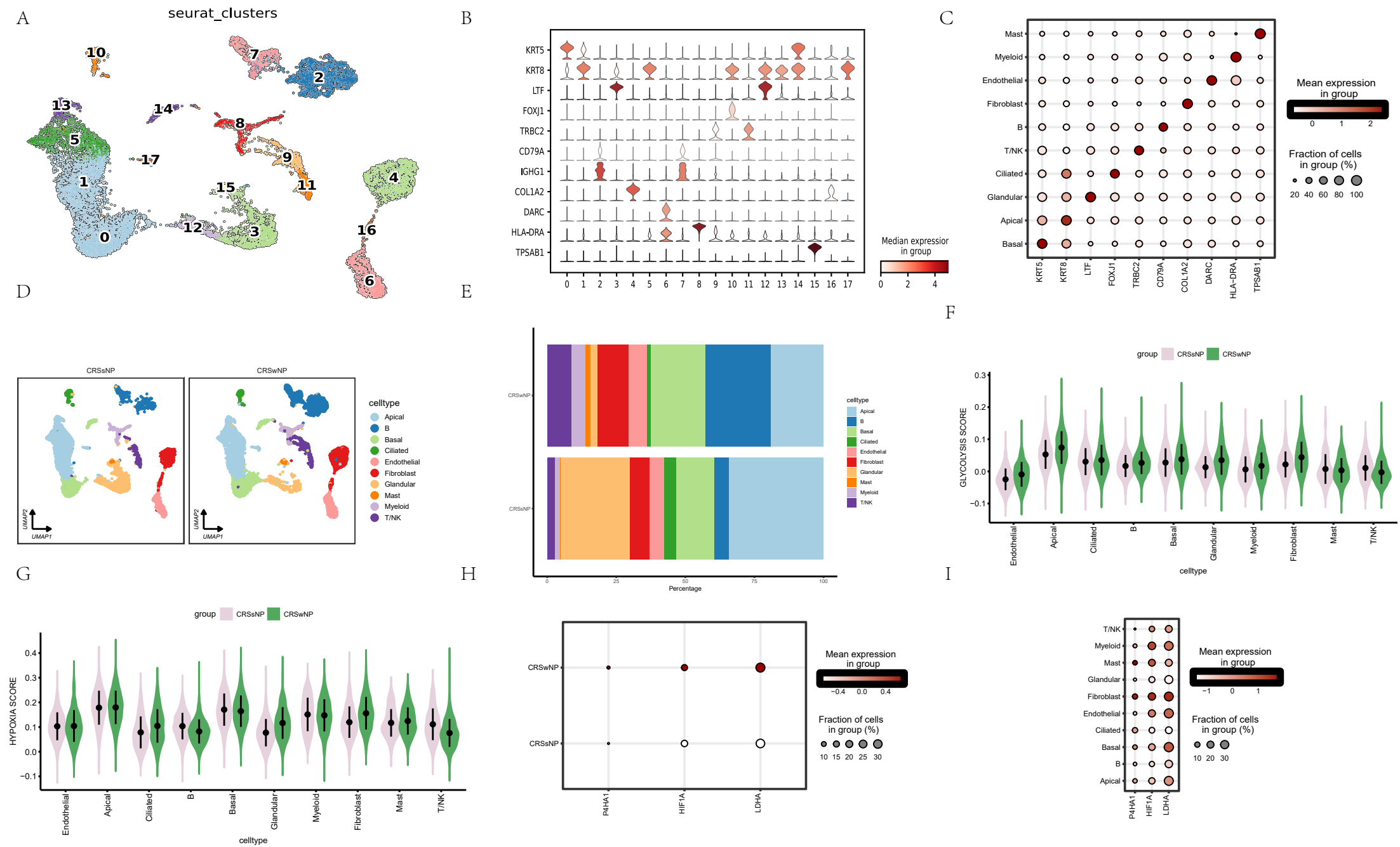
FIGURE 7 | (A) umap projection of all cells,resolution=0.8. (B) Violin plot depicts distributions of cell type marker genes in each cluster using density curves. (C) Dot plot of cell type marker genes. (D) umap projections for the CRSsNP and CRSwNP groups, respectively. (E) Cell proportion of each cluster of sample group. (F) Glycolysis pathway scores for CRSsNP and CRSwNP groups in all celltype. (G) Hypoxia pathway scores for CRSsNP and CRSwNP groups in all celltype. (H,I) Dot plots of P4HA1, HIF1A and LDHA gene expression.
