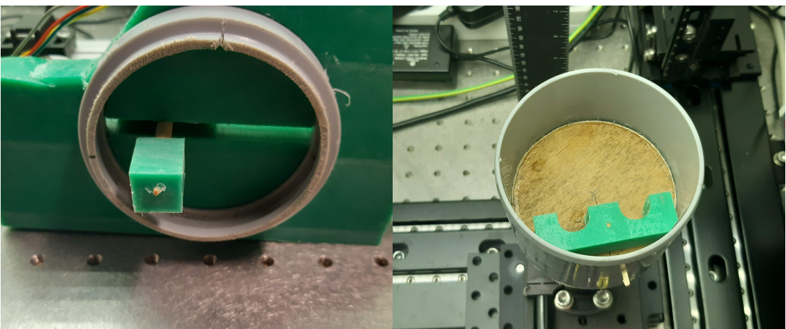
Figure 2. Interior parts of STEMPO phantom visible in the X-ray projections. On the left: moving HDPE block. On the right: boundary pipe and a static HDPE detail.
