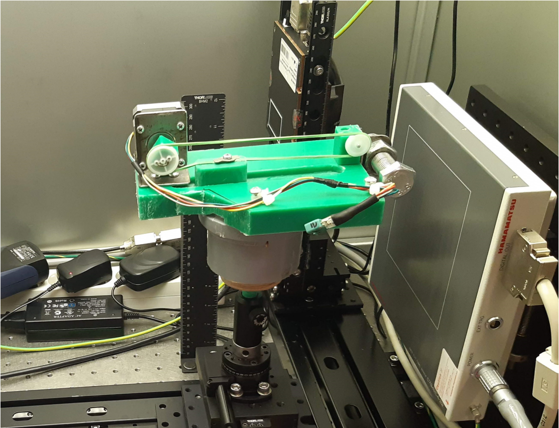
Figure 1. STEMPO phantom inside the micro-CT device. The static and dynamic objects of interest inside the pipe are not visible from the outside.
