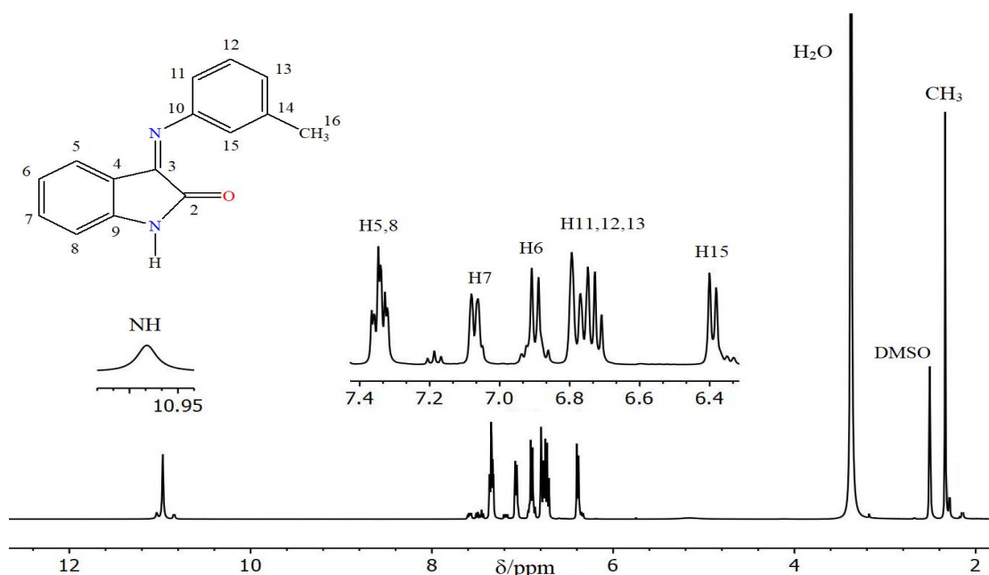
Fig 1 1 H NMR spectrum for HL1 in DMSO-d 6 at 20 °C
