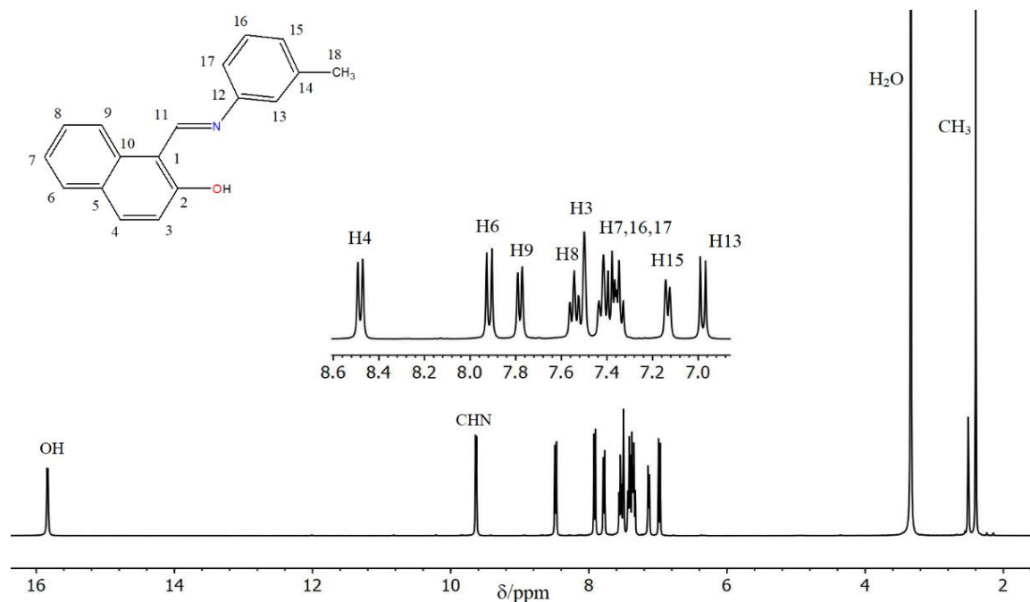
Fig 2 ^1\text{H} NMR Spectrum for HL2 in \text{DMSO-d}_6 at 20\text{ }^\circ\text{C}
