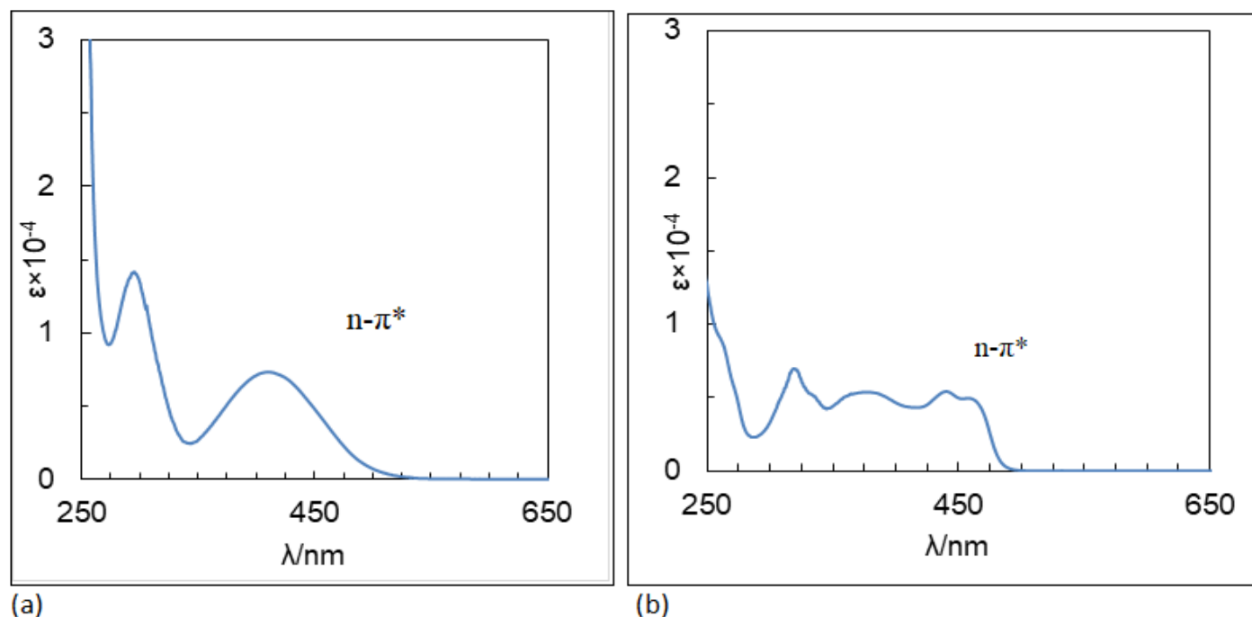
Fig 3 Experimental Spectrum for HL1 (a) and HL2 (b) ( ca. 0.10\text{ mM} ) in chloroform at 25\text{ }^\circ\text{C}
