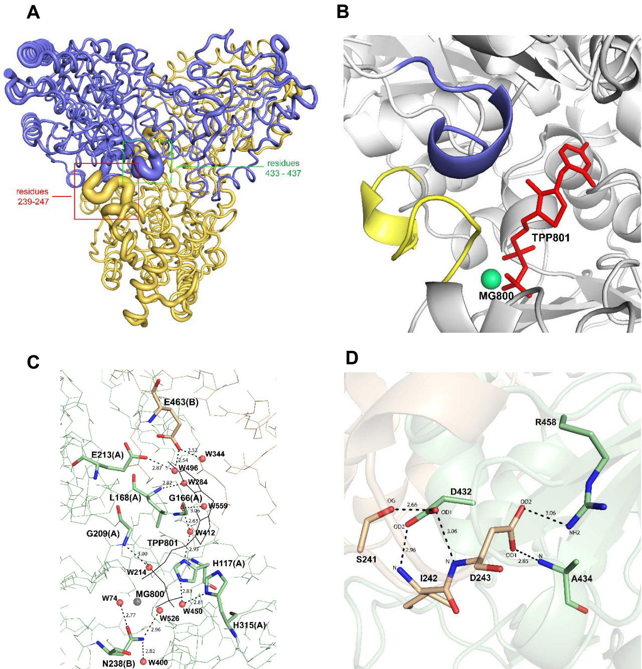
Fig. 6. Comparison between CrTK_{apo} and CrTK_{TPP/Mg} structures. (A) Representation of the CrTK_{apo} dimer structure. The thickness is correlated to the atom thermal factor (B-factor). The highlighted protein regions (239-247 and 433-437) are disordered and flexible. (B) CrTK_{TPP/Mg} structure reveals that the same protein regions have an ordered conformation and interact with TPP and Mg^{2+} . (C) CrTK_{apo} active site structure shows that water molecules occupy the position of TPP in CrTK_{TPP/Mg} structure (represented by grey thin lines for TPP and sphere for Mg^{2+} ) and stabilize catalytic residues by hydrogen bonds. (D) Dimer interface in CrTK_{TPP/Mg} structure showing the interactions between the residues belonging to
