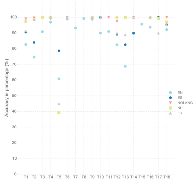
Figure 5: Language-based accuracy based on the TF features and the agreement-based retraining technique: left) using just the agreed samples for training (CL(i)), and right) using the agreed and the initial training samples for training (CL(ii)).
