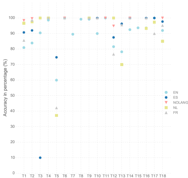
Figure 5: Language-based accuracy based on the TF features and the agreement-based retraining technique: left) using just the agreed samples for training (CL(i)), and right) using the agreed and the initial training samples for training (CL(ii)).
