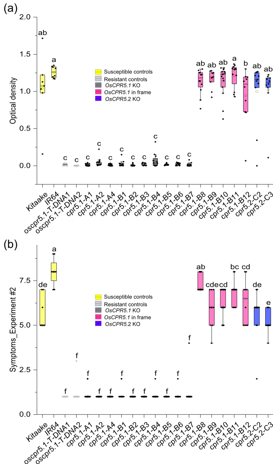
Figure 3. RYMV resistance evaluation in oscp5.1 and oscp5.2 mutant lines after mechanical inoculation of BF1 isolate of RYMV. Four independent experiments were performed in green house conditions and only results of experiment 2 are reported here. (a) Virus load in plants was detected using ELISA on leaf samples collected two weeks after inoculation. (b) Symptoms two weeks after inoculation were recorded using a disease scale ranging from 1 to 9. Boxes extend from 25th to 75th percentiles and display median values as center lines. Whiskers plot minimum and maximum values, asterisks indicate individual data points and detected by one-way ANOVA followed by Tukey's test, different letters indicate significant differences ( p < 0.05 ).
