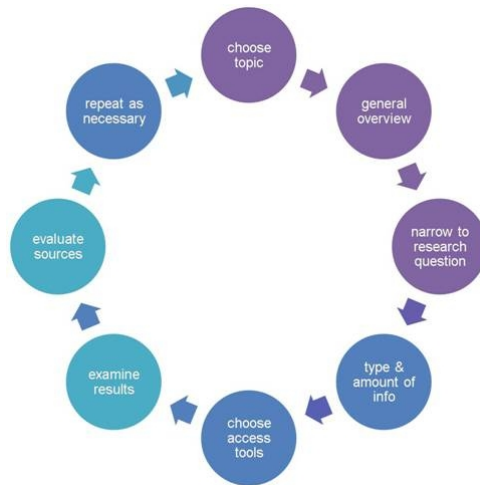
Fig. 5. Research Process
