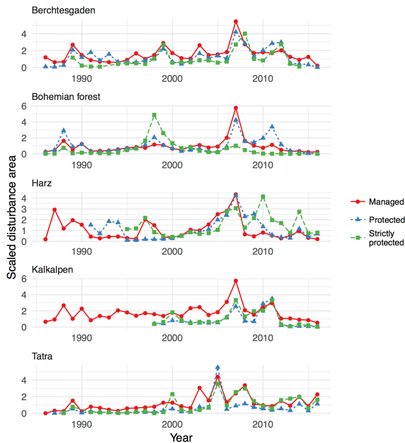
Figure 4: Temporal disturbance dynamics. Note that for facilitating comparisons between management zones, disturbances areas were scaled to units of standard deviation.
