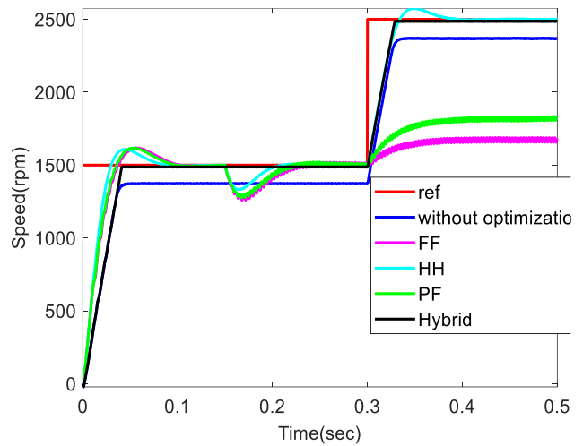
Fig.5 Speed response curve for case 2
