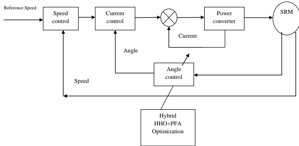
Fig.1: Block diagram of SRMD system
