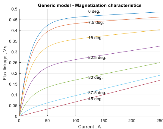
Fig.2 Magnetization characteristics of proposed SRMD
