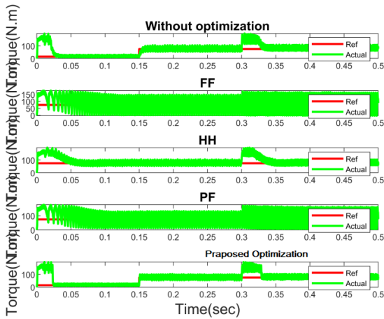
Fig.(7) Torque response of SRM motor for case 1
