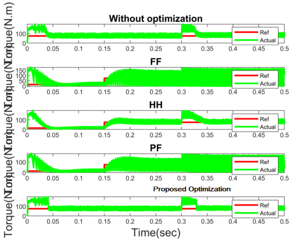
Fig.(8) Torque response of SRM motor for case 1
