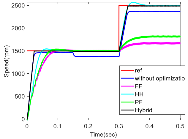
Fig.4 Speed response curve for case 1
