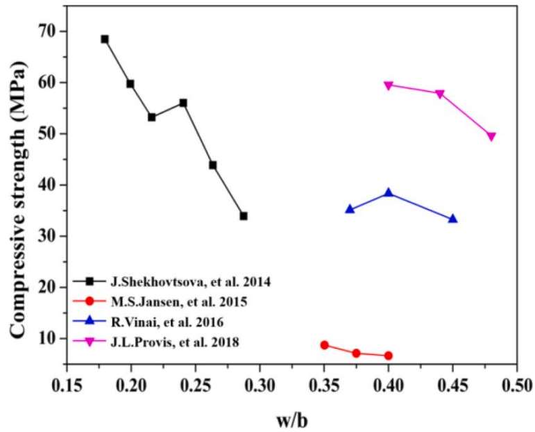
Figure 4-3 Effect of water/binder ratio on the compressive strength of slag and fly ash-based alkali-activated materials [244]
