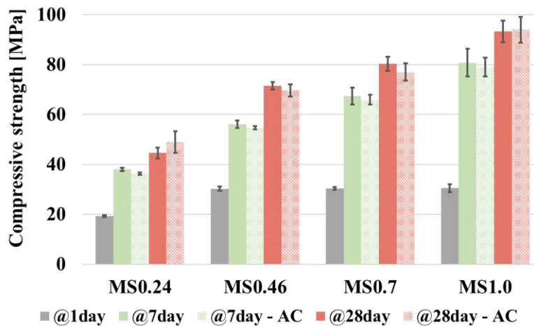
Figure 5-15 Compressive strength development of repair mortar with different molar ratios under pre-defined curing regimes
