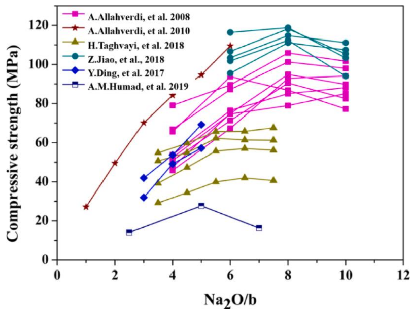
Figure 4-4 Effect of Na 2 O/binder ratio on the compressive strength of slag and fly ash-based alkali-activated materials [244]
