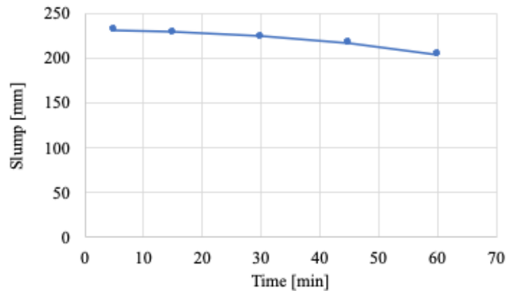
Figure 4-2 Slump retention of one type of URBCON concrete over time
