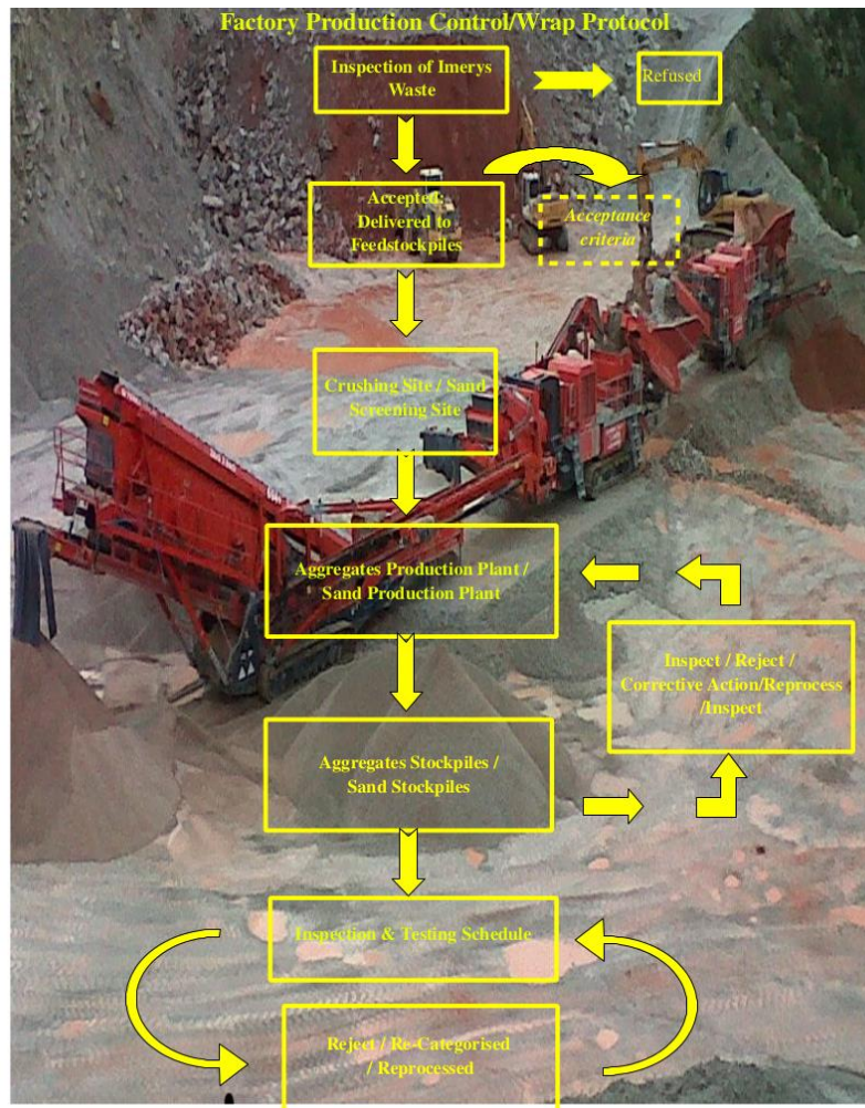
Figure 2-27 Production flow aggregates from kaolin waste (courtesy of Brookland Sand and Aggregates Ltd. UK)
