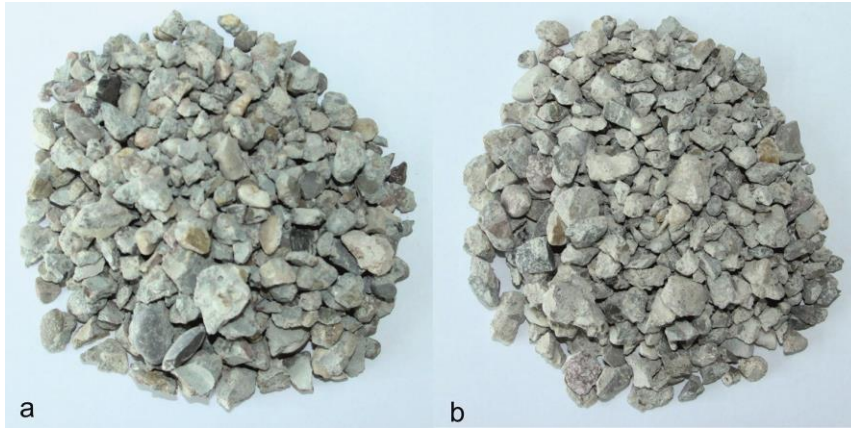
Figure 2-20 Recycled aggregates extracted from URBCON-concrete slabs. (a) URBCON-concrete made by natural aggregates (b) URBCON-concrete made by recycled aggregates type 1
