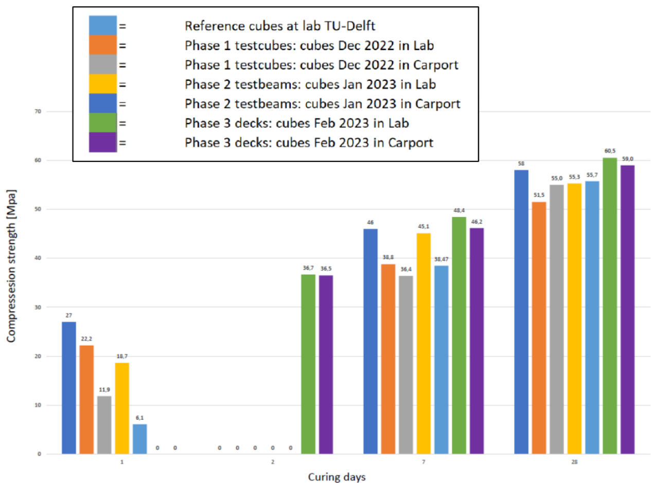
Figure 9-4 Strength development of test cubes
