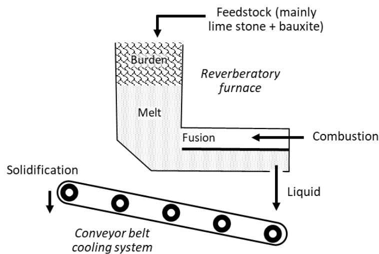
Figure 2-5 Reverberatory furnace (adapted from [41])
