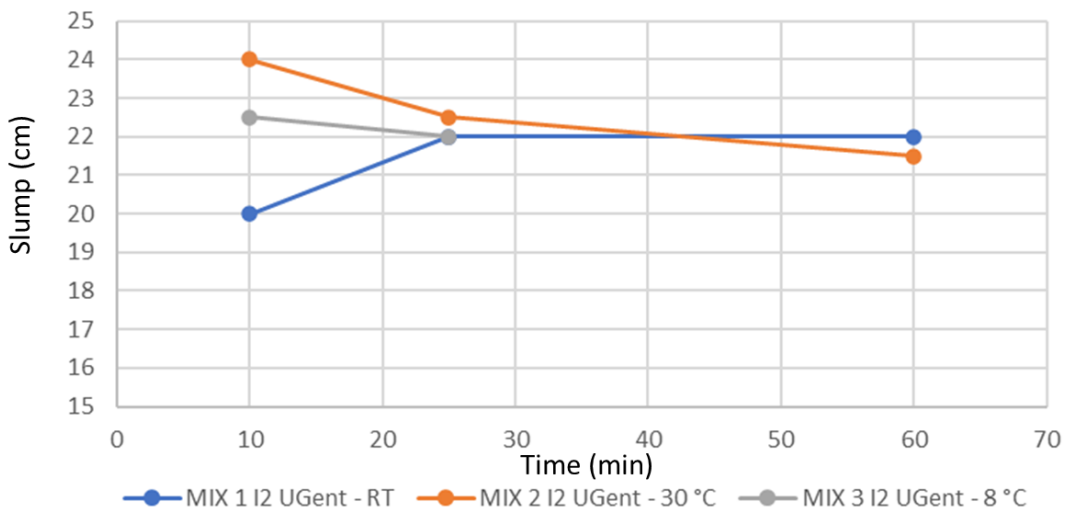
Figure 5-3 Slump of MIX1, MIX2 and MIX3 after 10, 25 and 60 min after mixing
