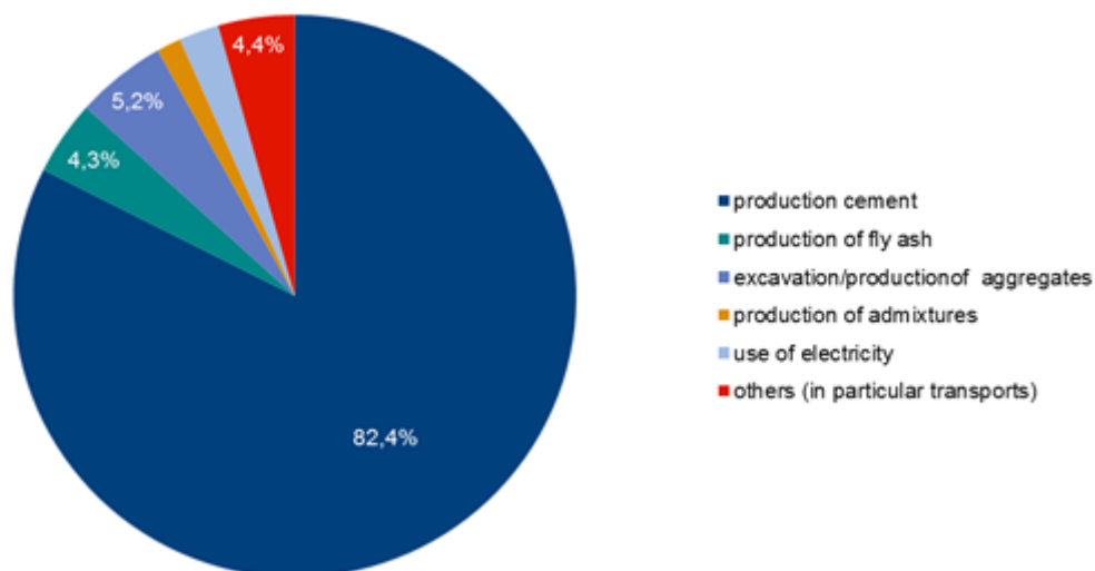
Figure 7-6 Concrete production: main influence factors on Global Warming Potential (Germany: IZB C25/30) [362]
