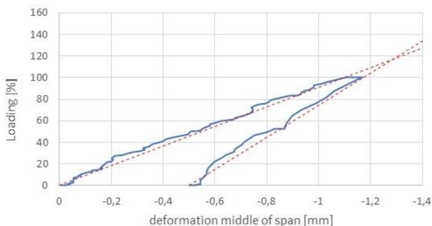
Figure 9-8 Measured deformation at the middle of the span
