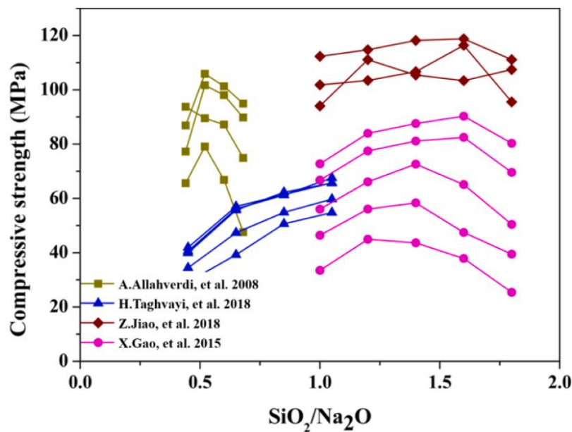
Figure 4-5 Effect of SiO 2 /Na 2 O ratio on the compressive strength of slag and fly ash-based alkali-activated materials [244]
