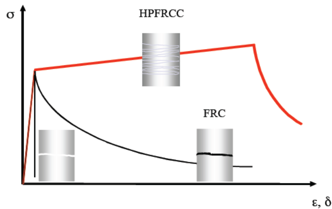
Figure 5-13 Tensile response of normal concrete, fibre-reinforced concrete (FRC) and high-performance fibre-reinforced cementitious composites (HPFRCC) under uniaxial tension [350]
