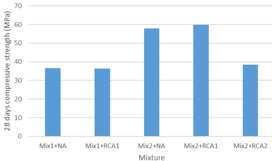
Figure 5-2 Compressive strength of Mix1 and Mix2 with normal coarse aggregates (NA) and recycled aggregates type 1 (RCA1) and type 2 (RCA2) after 28 days
