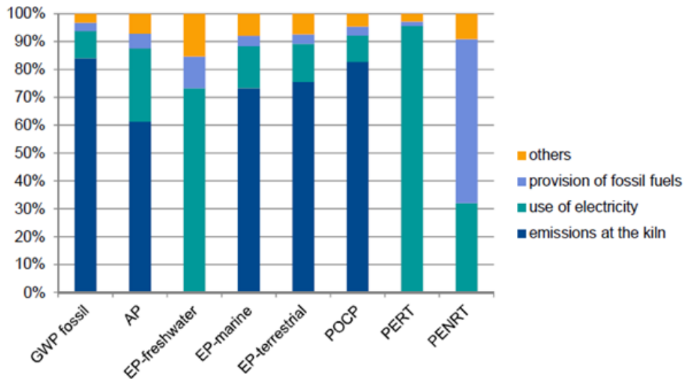
Figure 7-3 Cement production: main influence factors on the values of selected environmental indicators (CEMBUREAU representative CEM II) [363]
