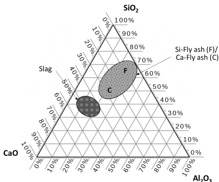
Figure 3-1 Chemical compositions of different fly ashes and blast furnace slags reported in the literature, accounting for the main reactive oxides (adapted from [42])
