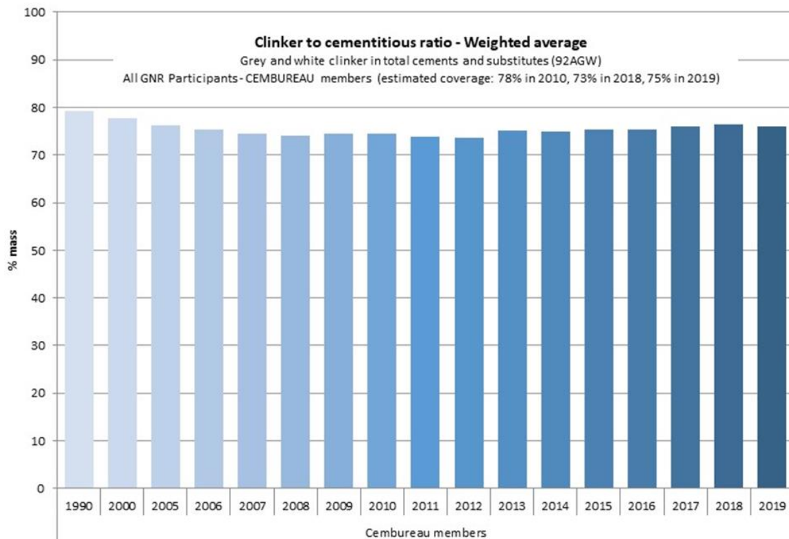
Figure 7-4 Clinker/cement ratio in CEMBUREAU member states 1990 until 2019 [363]
