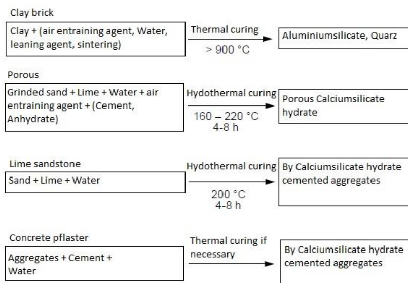
Figure 2-14 Comprehensive masonry materials scheme [65]
