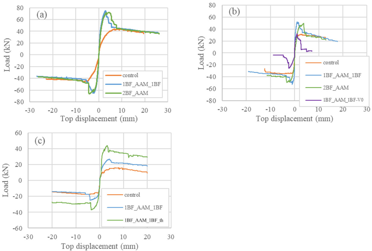
Figure 5-21 Hysteretic loop envelopes of AAM-based TRM strengthened walls for squat (a) and slender (b) specimens tested in-plane and specimens tested out-of-plane (c)
