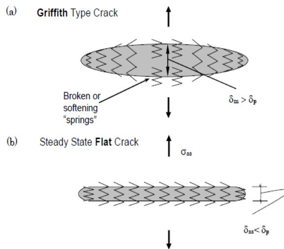
Figure 5-14 Steady state crack analysis [351]
