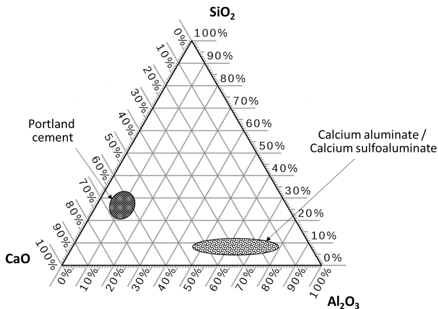
Figure 2-4 Zones of cementitious materials in the CaO-SiO 2 -Al 2 O 3 (adapted from [41])
