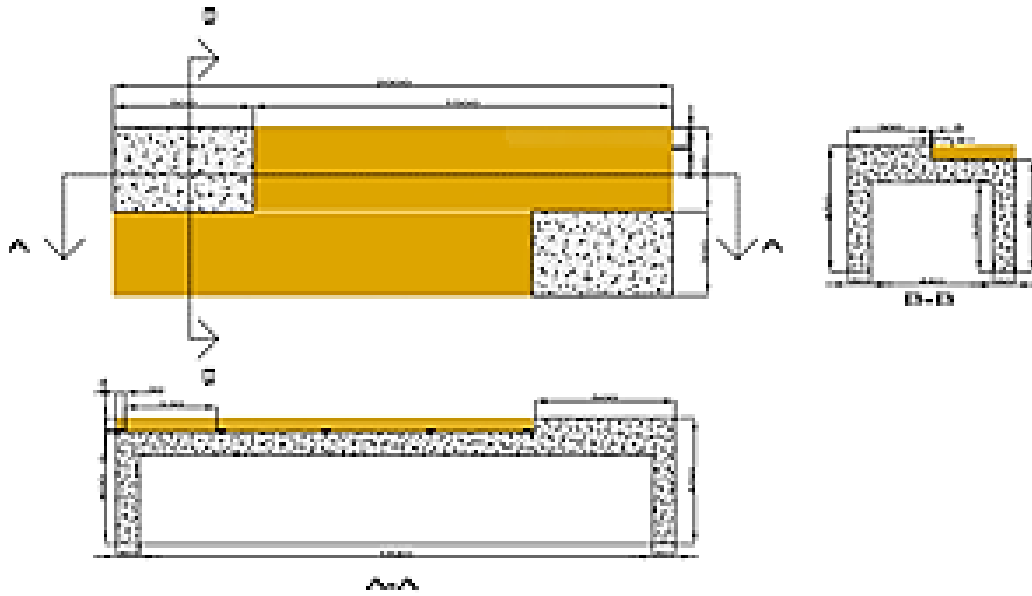
Figure 9-30 View and sections of the produced bench at RPTU
