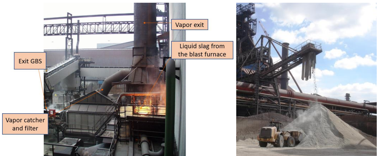
Figure 2-24 Slag granulation unit ex-blast furnace (left) and storing GBS (right)
