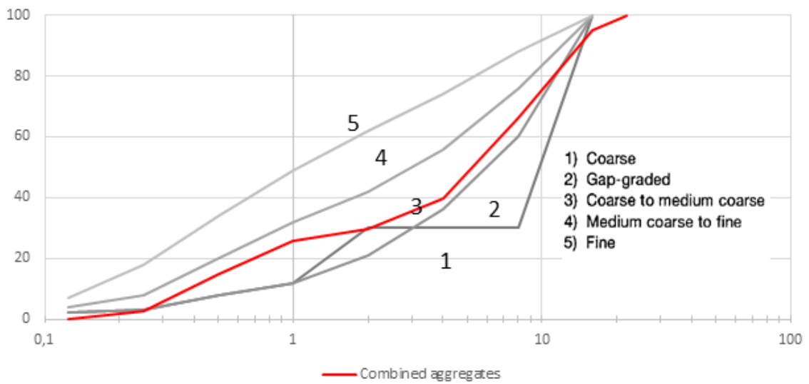
Figure 2-17 Grading of combined natural aggregates used in alkali-activated concrete mixtures
