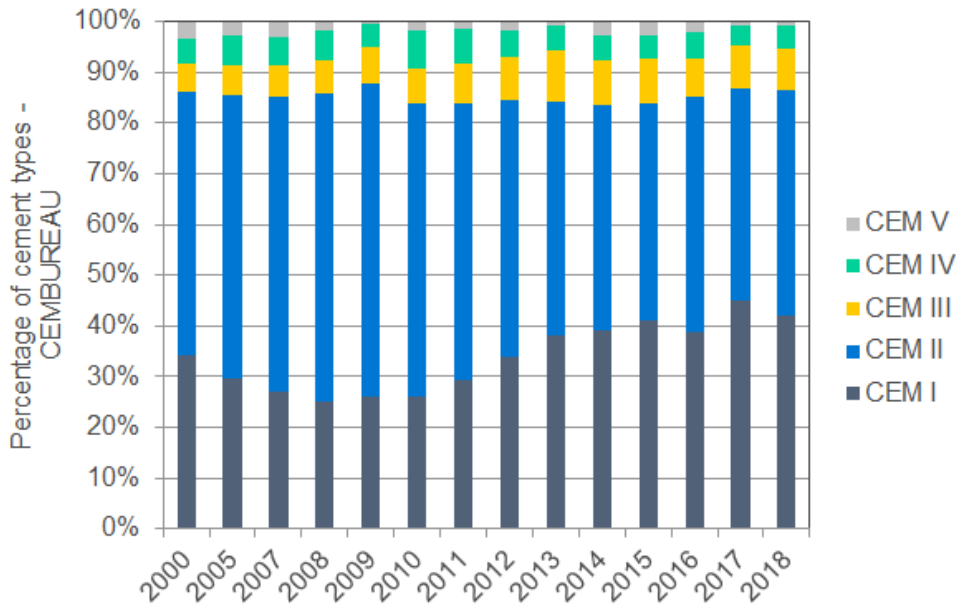
Figure 2-3 Domestic European cement delivery [32]
