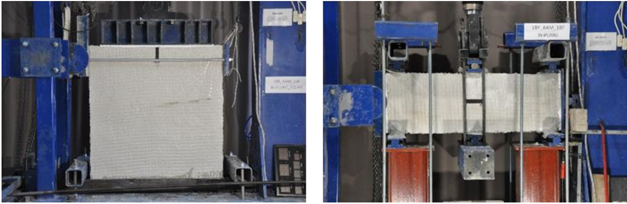
Figure 5-20 Test setups for in-plane tests of squat (left) and slender (right) walls
