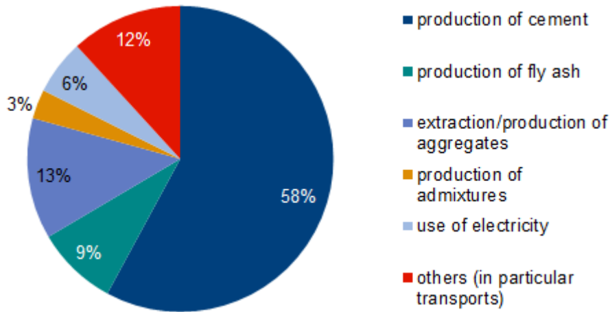
Figure 6-3 Contribution of different processes to the non-renewable primary energy use to produce average German C25/30 concrete [362]
