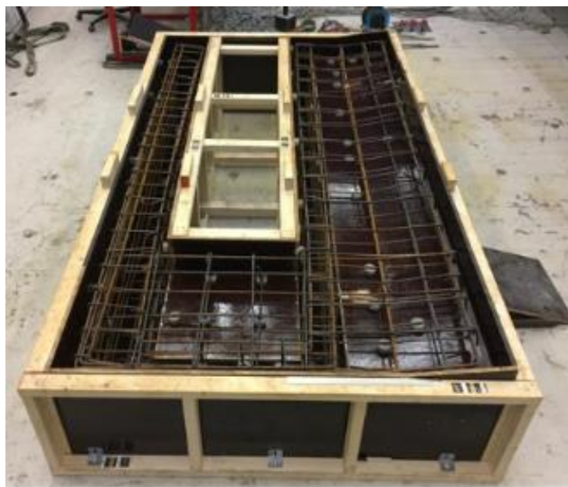
Figure 9-23 Mould and rebars for the bench [Z. Aldin, 2017, unpublished report]
