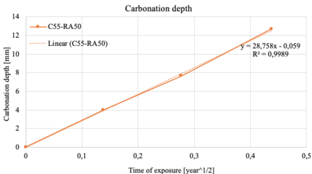
Figure 4-6 Carbonation depth of a type of URBCON concrete under an environment of 60% relative humidity and 1 % CO 2 concentration
