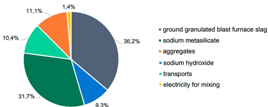
Figure 7-9 Influence of different components on the GWP (for mix RP1)
