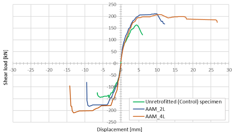
Figure 5-22 Shear load-displacement hysteretic loop envelopes
