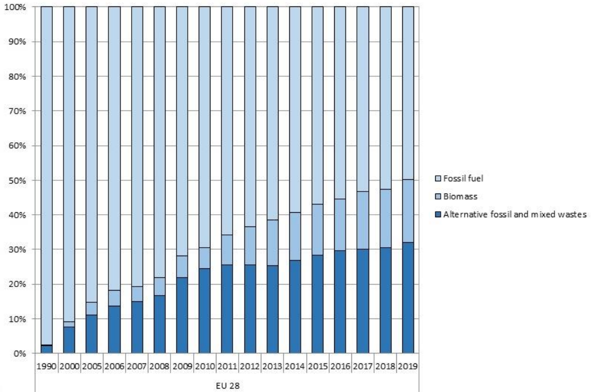
Figure 6-5 Thermal energy consumption (excluding drying of fuels), weighted average [364]
