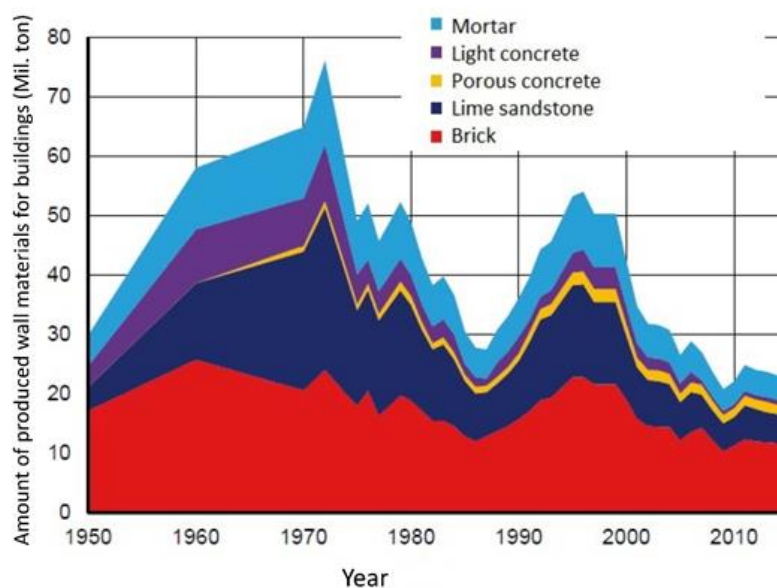
Figure 2-13 Annual production of masonry materials in Germany [61][66]-[68]
