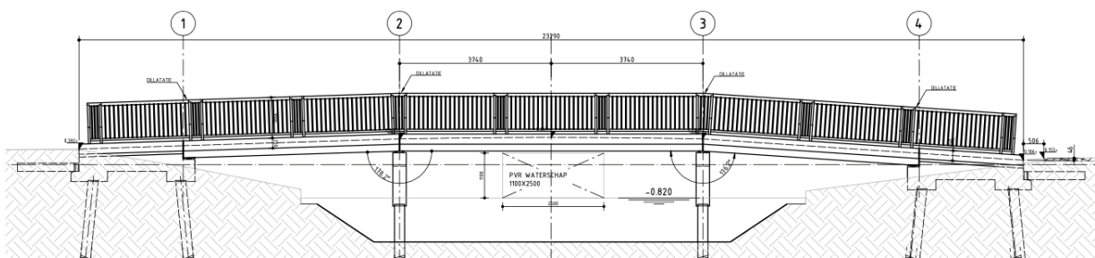
Figure 9-1 Overview pilot bridge at Rotterdam
