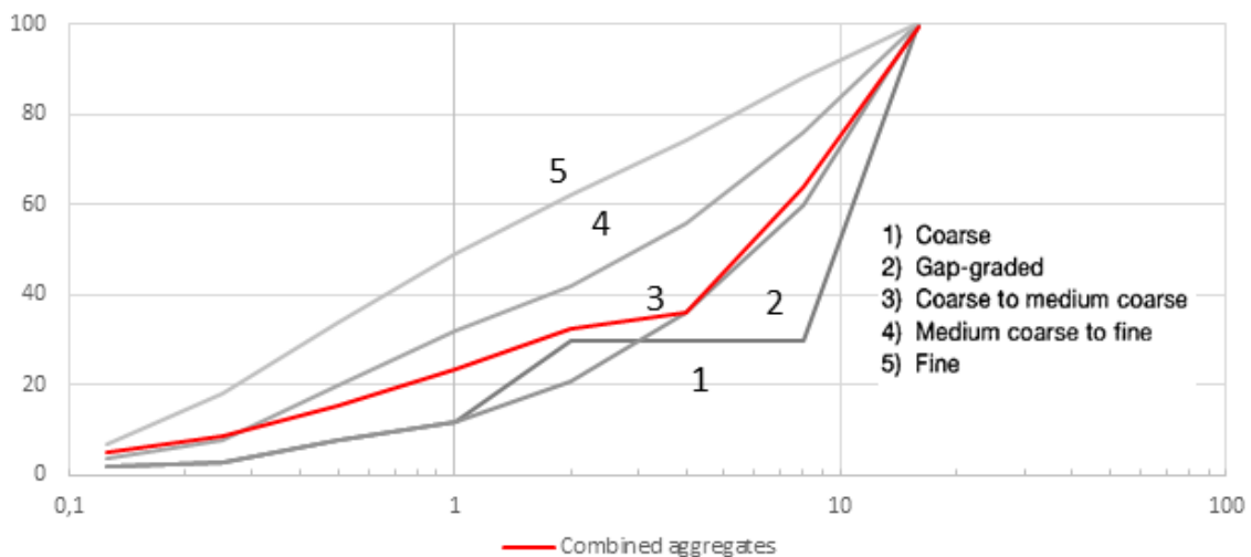
Figure 2-19 Grading of combined recycled aggregates used in alkali-activated concrete mixtures
