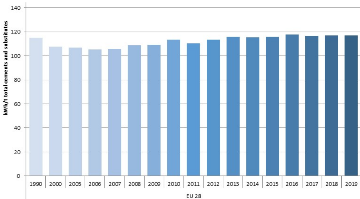
Figure 6-6 Cement plant power consumption (weighted average) [366]
