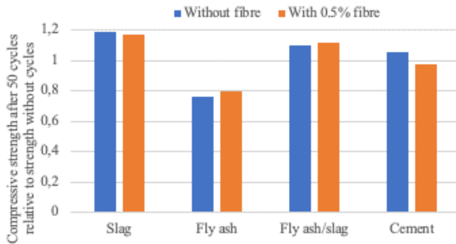
Figure 4-10 Compressive strength of AAM and PC mortar with/without polypropylene fibres after 50 freeze-thaw cycles in water relative to original strength before cycling (adapted from [283])
