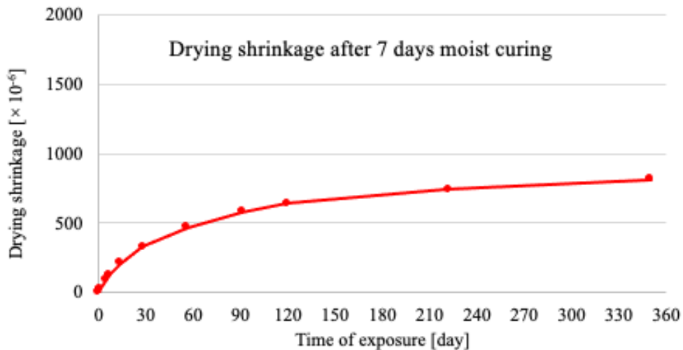
Figure 4-12 Drying shrinkage of a type of URBCON concrete under 50% relative humidity at 20°C
