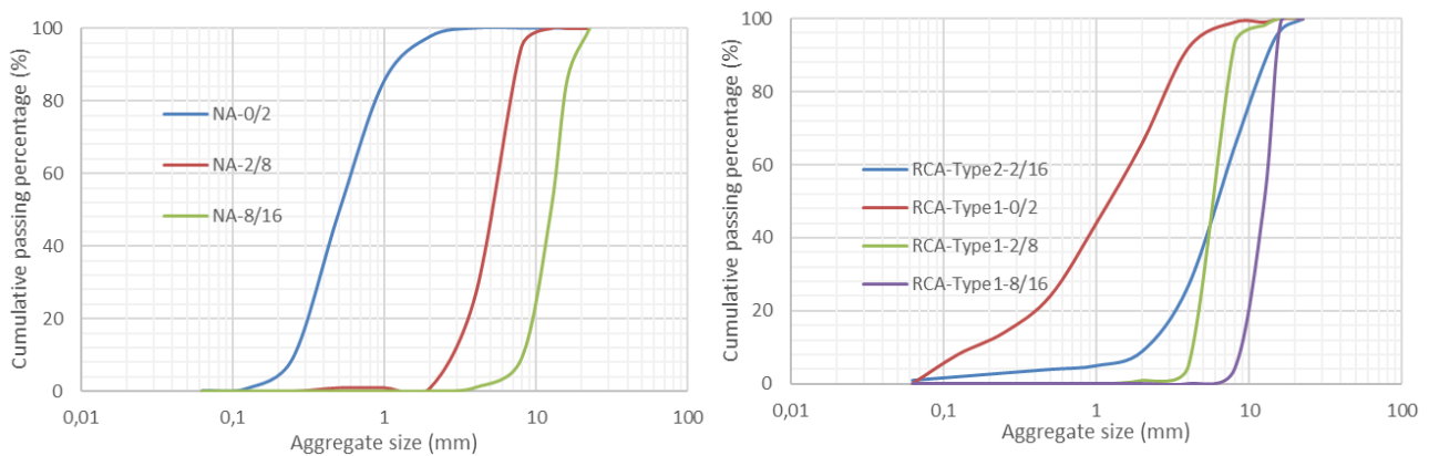
Figure 2-15 Particle size distribution of natural (left) and recycled aggregates (right)
