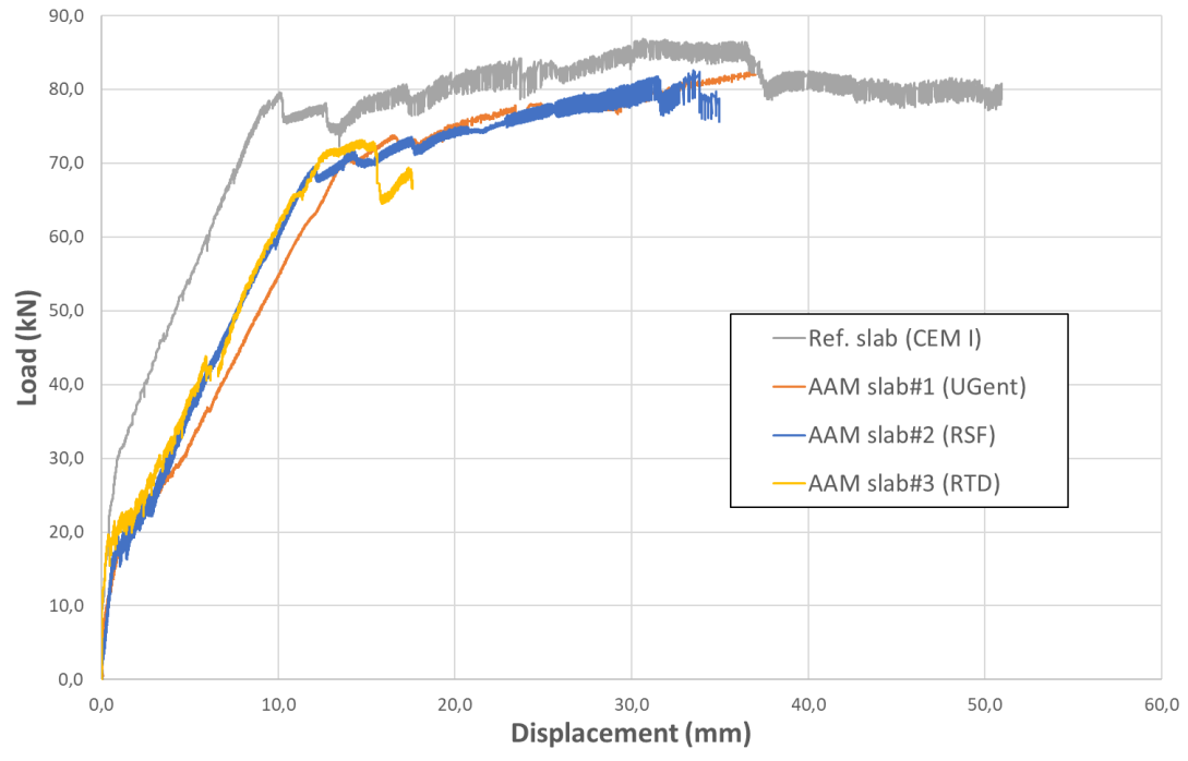
Figure 5-9 Shear tests on slabs: load-deflection response
