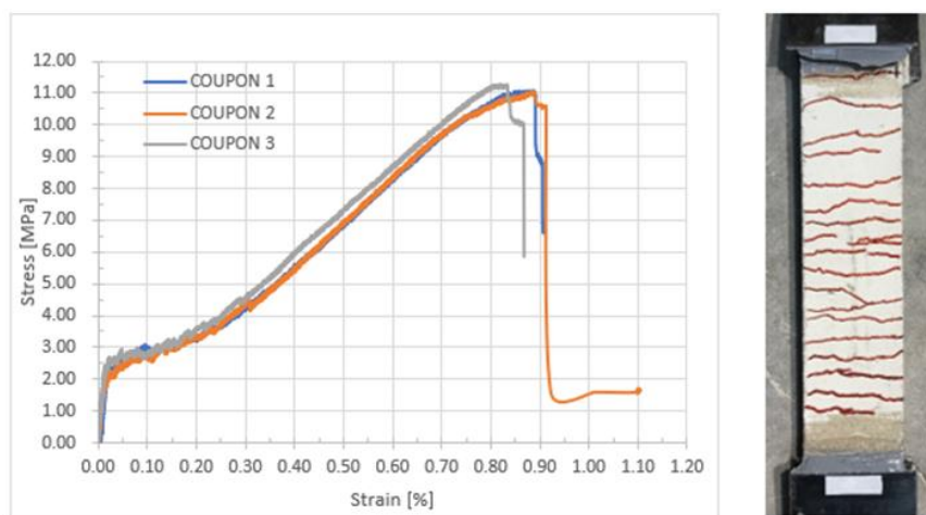
Figure 5-19 Stress-strain behaviour of AAM TRM tensile coupons
