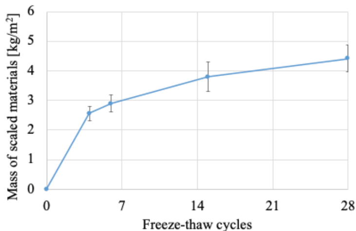
Figure 4-9 Freeze-thaw resistance of a type of URBCON concrete following CDF testing method
