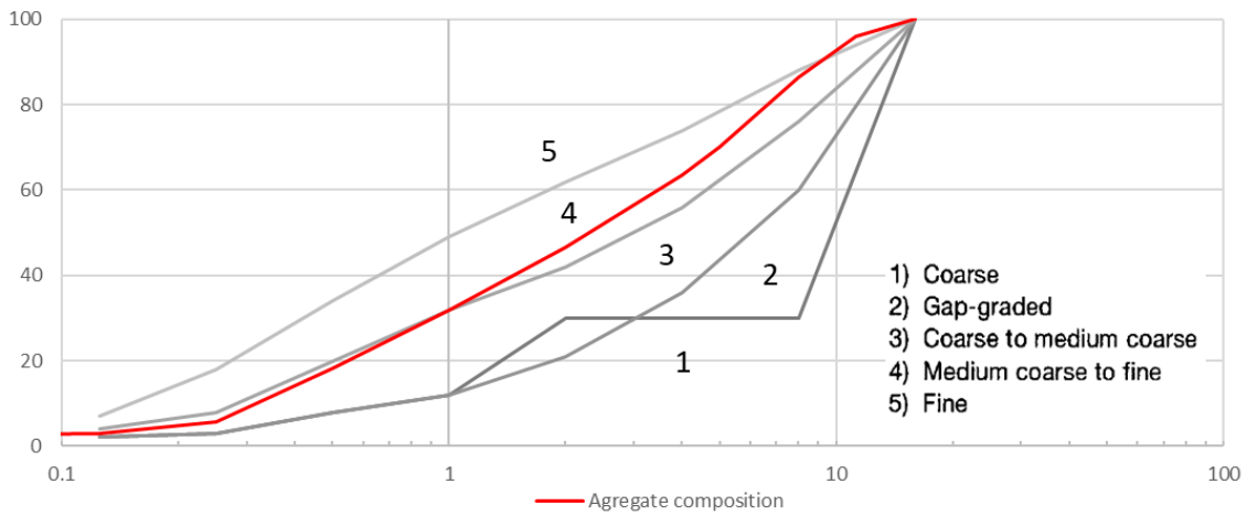
Figure 2-21 Grading of combined URBCON recycled aggregates (whereby the recycled aggregates came for URBCON concrete produced with 100% natural aggregates)
