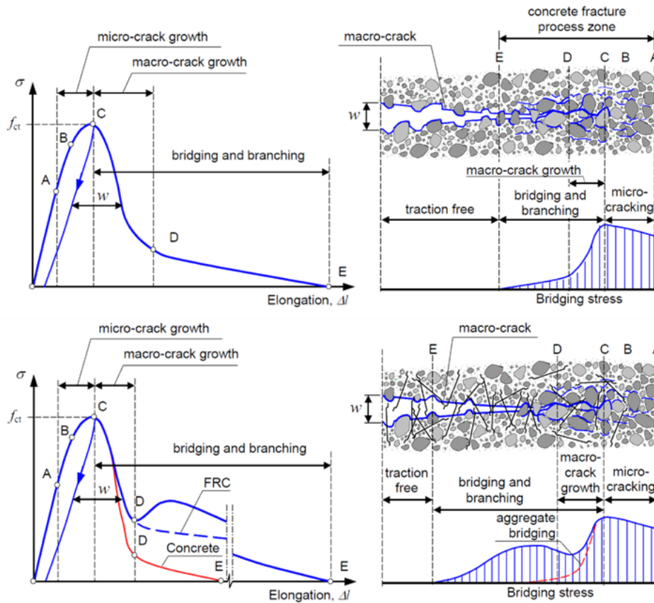
Figure 5-11 Crack propagation and related stress-strain curve in plain and fibre-reinforced [347]
