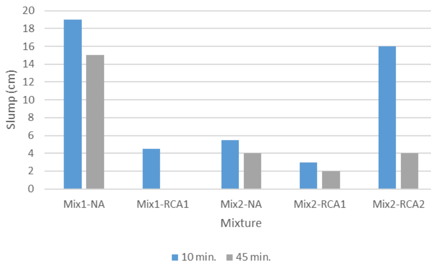
Figure 5-1 Slump of Mix1 and Mix2 with normal coarse aggregates (NA) and recycled concrete aggregates type 1 (RCA1) and type 2 (RCA2) after 10 and 45 min
