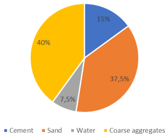
Figure 6-1 Raw materials for concrete in weight percentage
