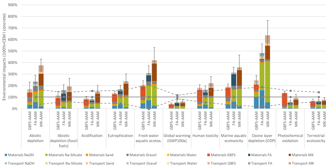
Figure 7-7 Environmental impacts of AAM mixes, compared to PC concrete including quantified variability and uncertainty
