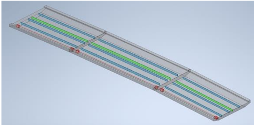
Figure 9-2 Monitoring system used for the pedestrian bridge (in blue the strain measuring loops, in green the temperature loop)
