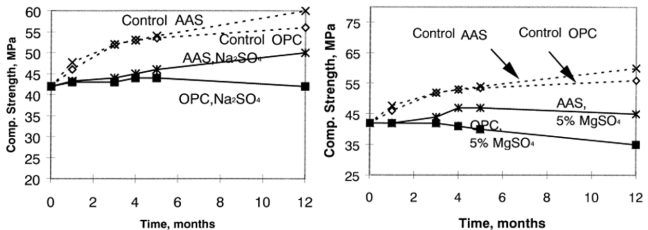
Figure 4-8 Compressive strength of PC concrete and AAS concrete subjected to Na_2SO_4 (a) and MgSO_4 solution (b) [267]
