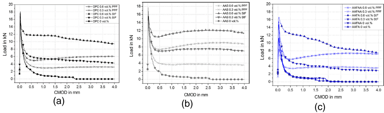
Figure 5-12 Load-CMOD relationships for PC (a), slag-based (b) and fly-ash-based (c) AAC, reinforced with steel and macro-PP fibres [349]
