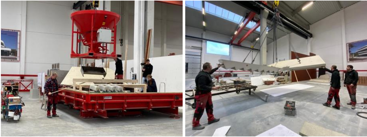
Figure 9-16 Production of precast elements for the staircase
