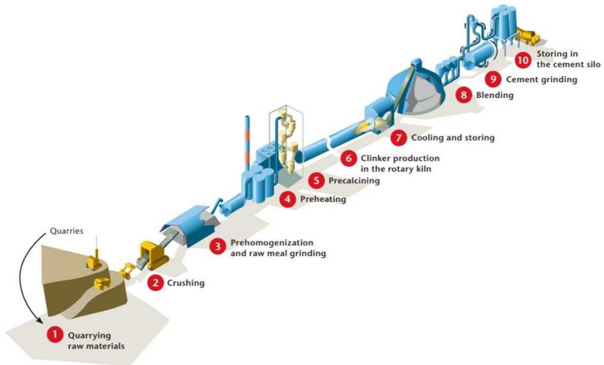
Figure 2-2 Schematic representation of the cement manufacturing process from quarry to dispatch [15]
