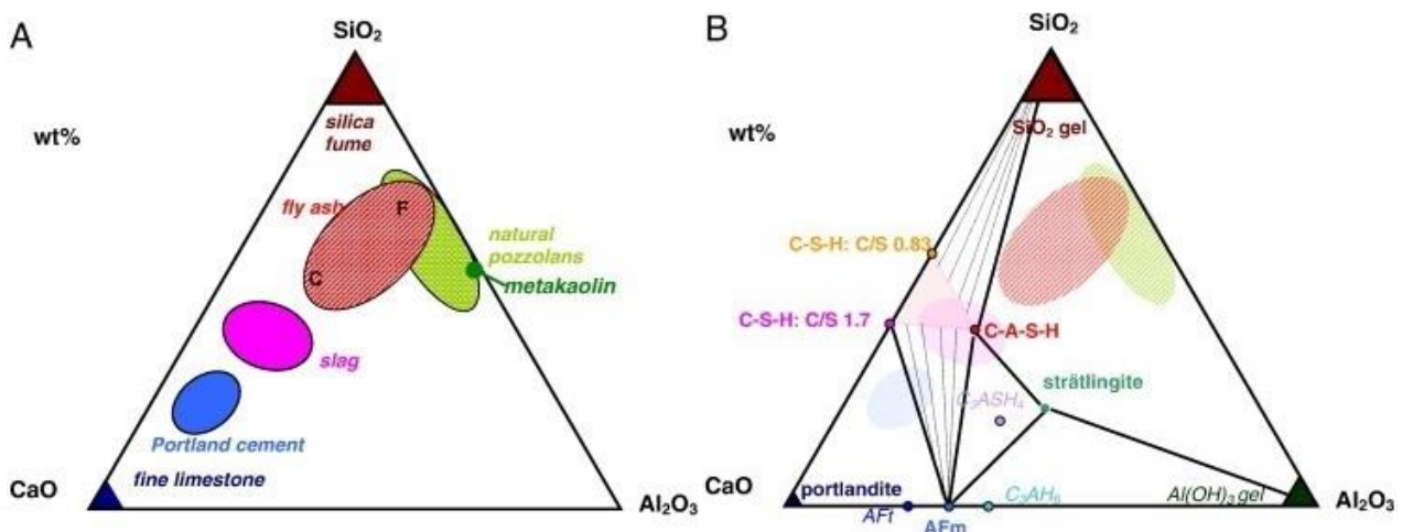
Figure 2-6 (A) CaO-Al 2 O 3 -SiO 2 ternary diagram of cementitious materials; (B) hydrate phases in the CaO-Al 2 O 3 -SiO 2 system (adapted from [42])
