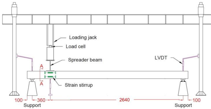
Figure 5-6 Test set-up (dimension in mm, not on scale) of flexural load tests (top) and shear load tests (bottom)
