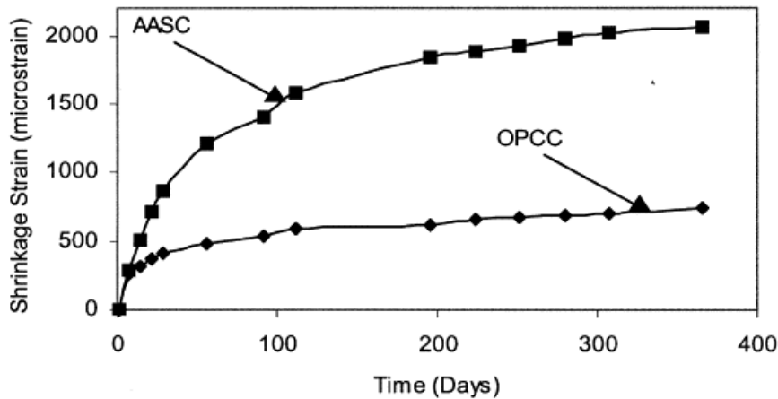
Figure 4-11 Drying shrinkage of PC and AAM concrete, exposed from day 1 onwards to 50% RH and 23°C. w/h=0.5 [299]
