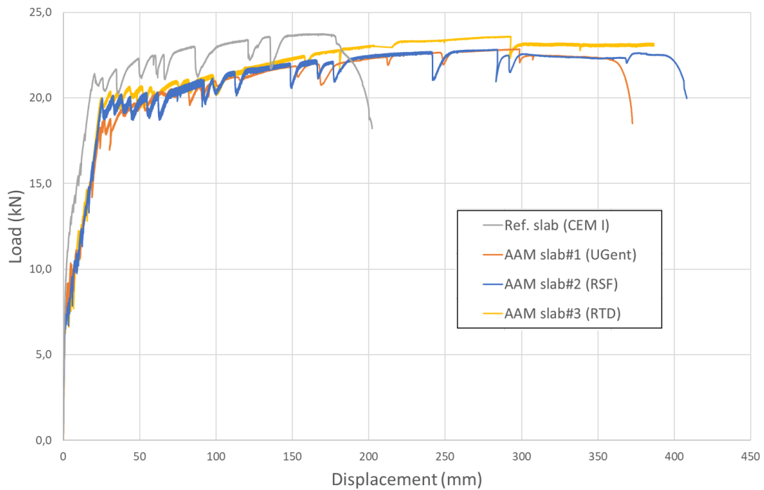
Figure 5-7 Flexural tests on slabs: load-deflection response
