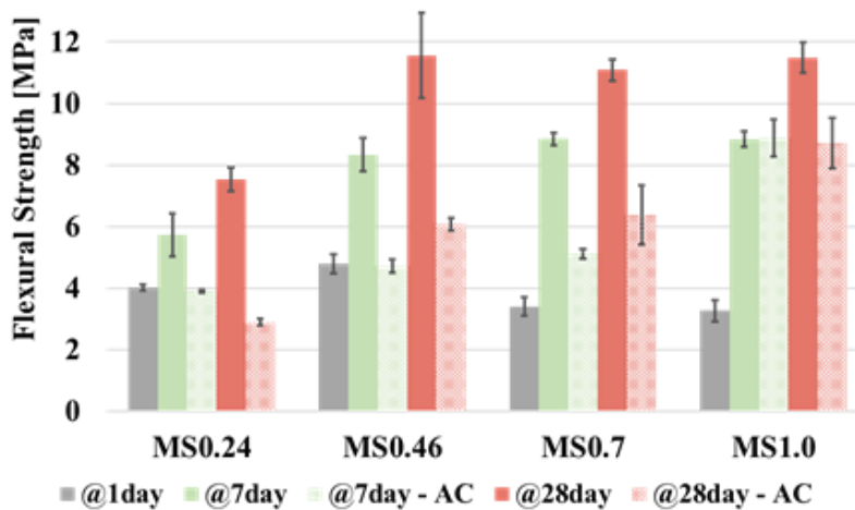
Figure 5-16 Flexural strength development of repair mortar with different molar ratios under pre-defined curing regimes
