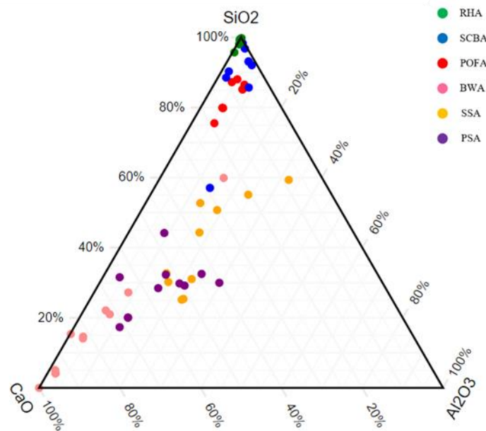
Figure 3-3 Distribution of the three main oxides in compositions of alternative precursors
