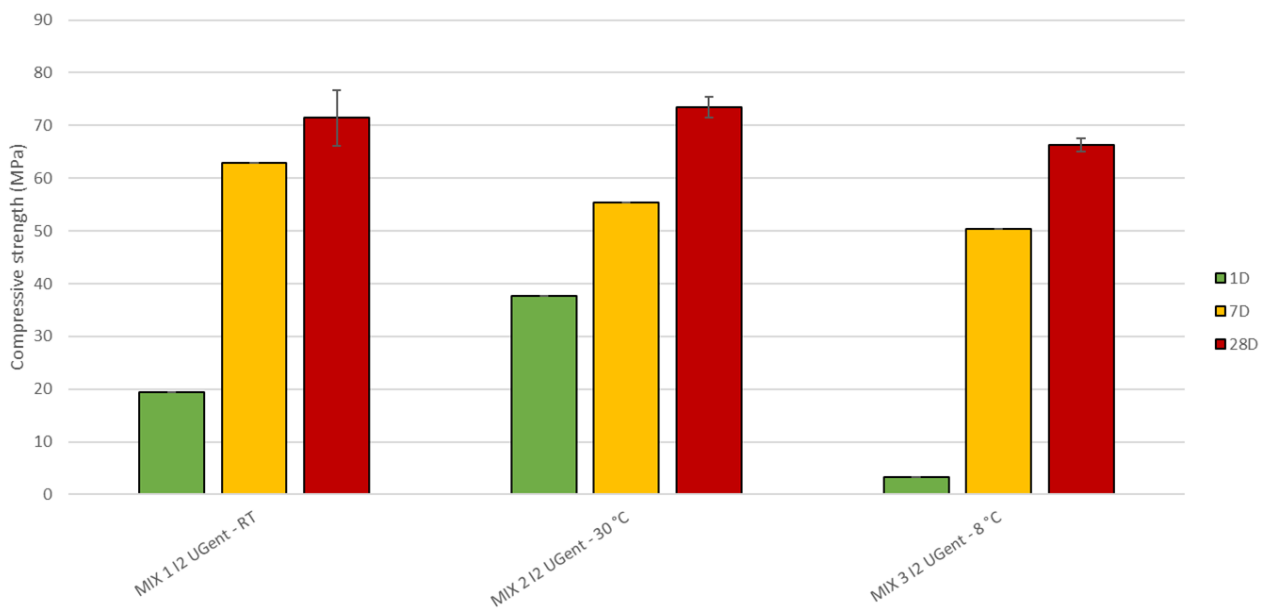
Figure 5-4 Compressive strength of MIX1, MIX2 and MIX3 after 1, 7 and 28 days
