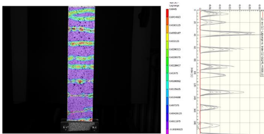
Figure 5-18 Cracking behaviour of AAM TRM tensile coupons
