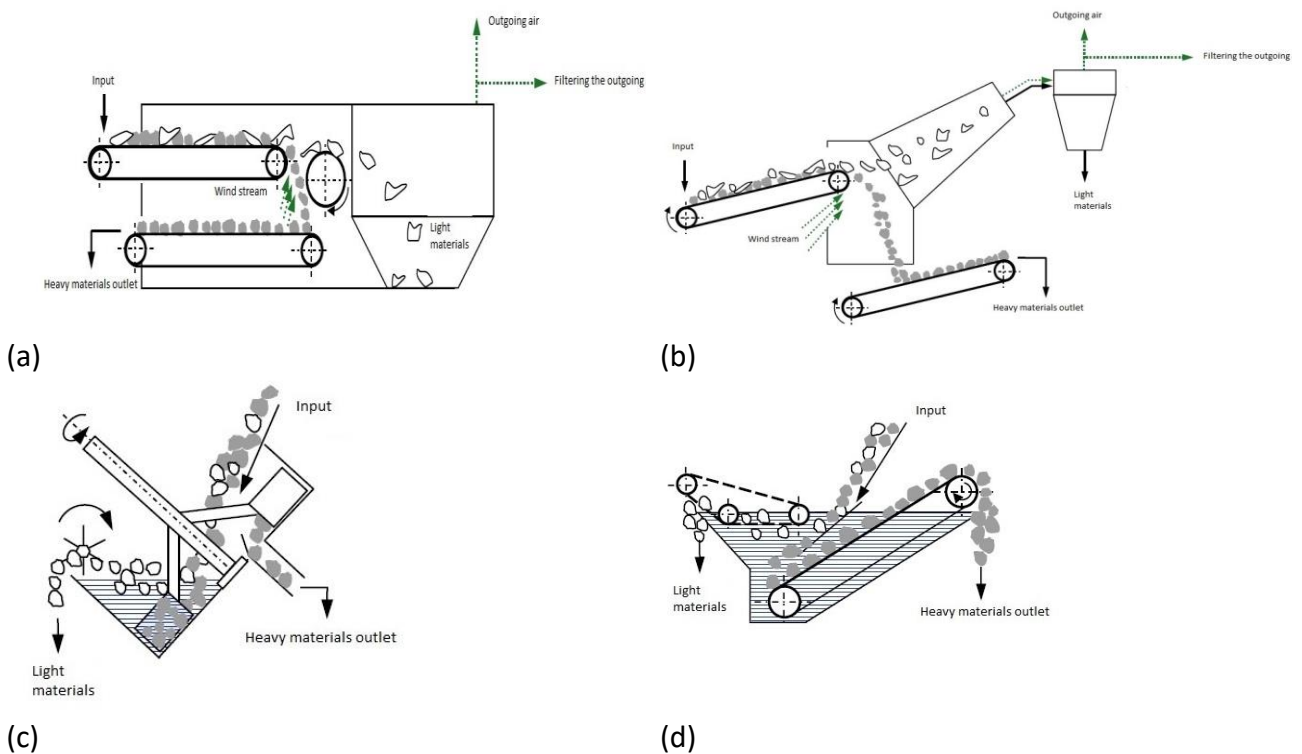
Figure 2-12 Sketches of two dried sorting machines for demolished materials (1st and 2nd) and two wet sorting machines (3rd and 4th) [61]
