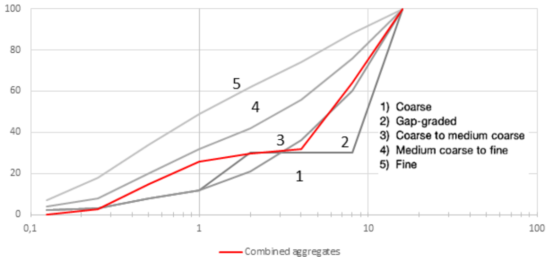
Figure 2-18 Grading of combined 70% recycled aggregates and 30% natural aggregates used in alkali-activated concrete mixtures
