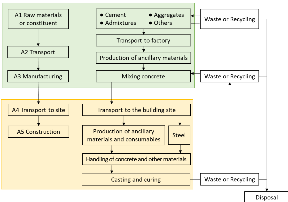
Figure 7-5 System boundaries of concrete production acc. to EN 16757 [371]
