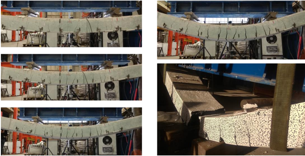
Figure 5-8 Flexural tests on slabs: observed crack development and slab failure
