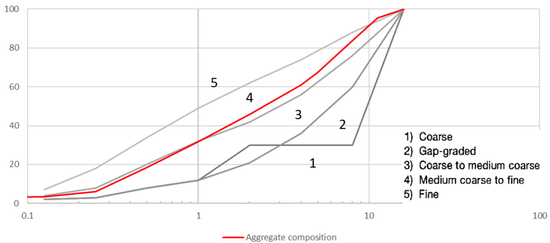
Figure 2-22 Grading of combined URBCON recycled aggregates (whereby the recycled aggregates came for URBCON concrete produced with 70% recycled concrete coarse aggregates)
