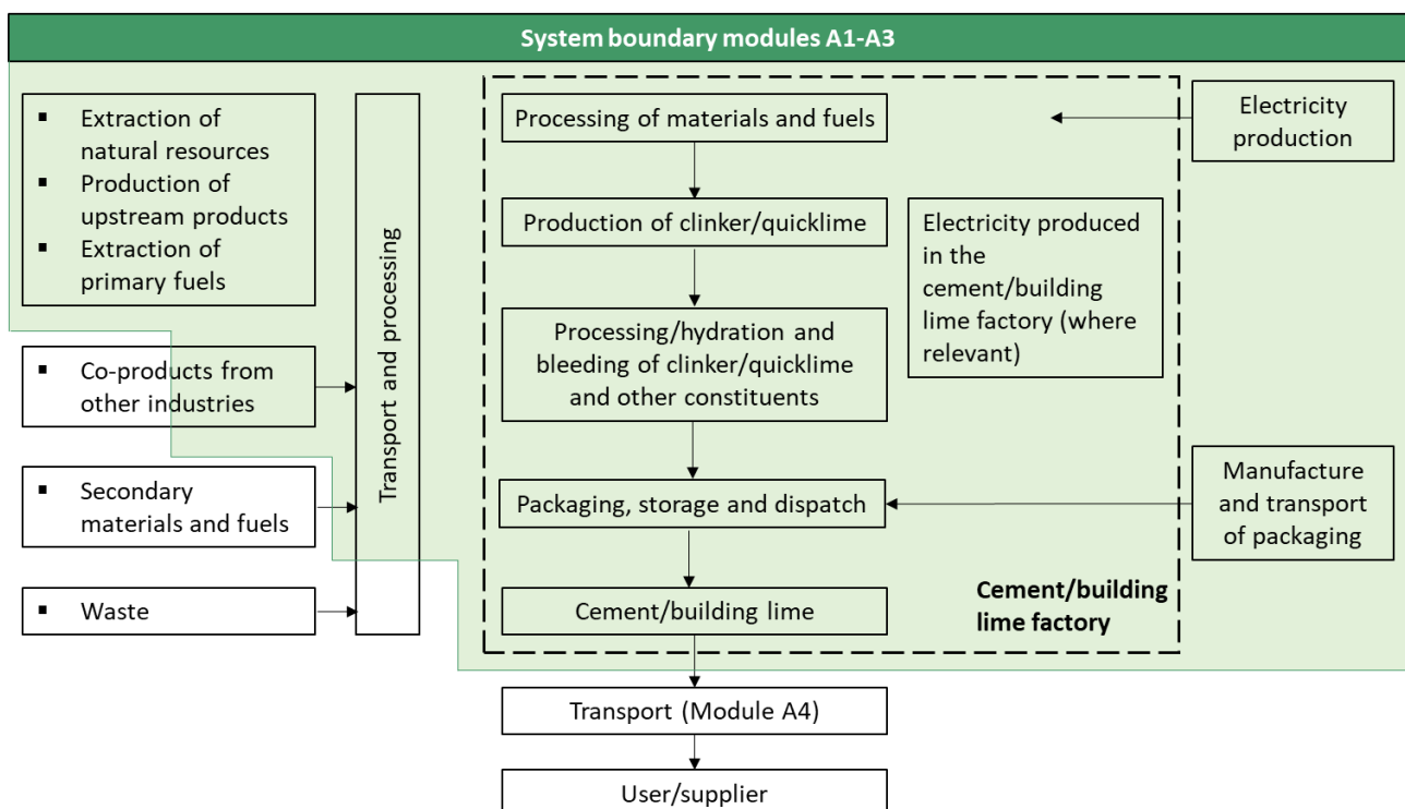
Figure 7-2 System boundaries of cement production acc. to EN 16908 [370]
