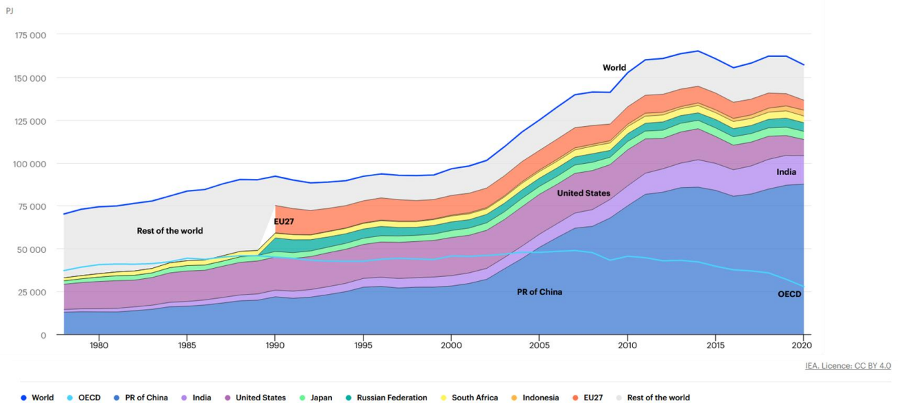
Figure 3-2 Profile of global coal consumption over time ( https://www.iea.org/data-and-statistics/charts/world-coal-consumption-1978-2020 )
