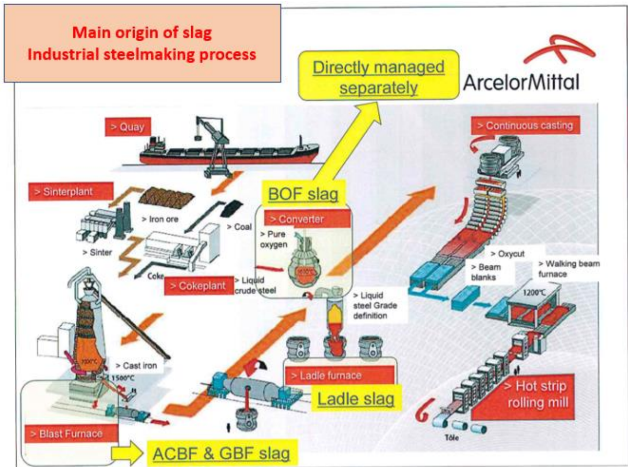
Figure 2-23 Process flow of steelmaking and main origin of slags in this process
