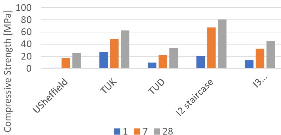
Figure 9-29 Compressive strength testing of modular bench elements
