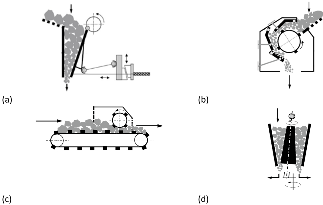
Figure 2-11 The sketches of the four most popular aggregates crushers (a) Swing-in jaw crusher, (b) Impact crusher, (c) Impact-roll crusher, (d) Cone crusher [61]
