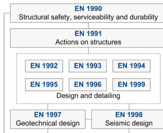
Figure 5-5 Links between Eurocodes [343]
