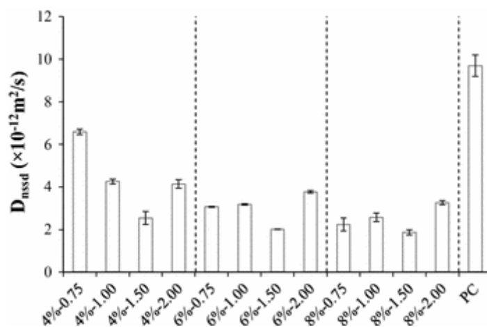
Figure 4-7 Non-steady state chloride diffusion coefficients of the concretes (“4%-0.75” stands for concrete made of 4% Na 2 O by mass of binder and the modulus 0.75 of water glass) [297]
