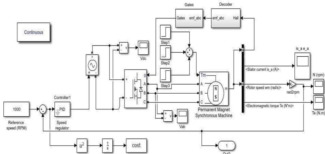
Figure 10: Model of BLDC motor with PSO
