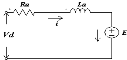
Figure 8: Per Phase equivalent of BLDC motor
