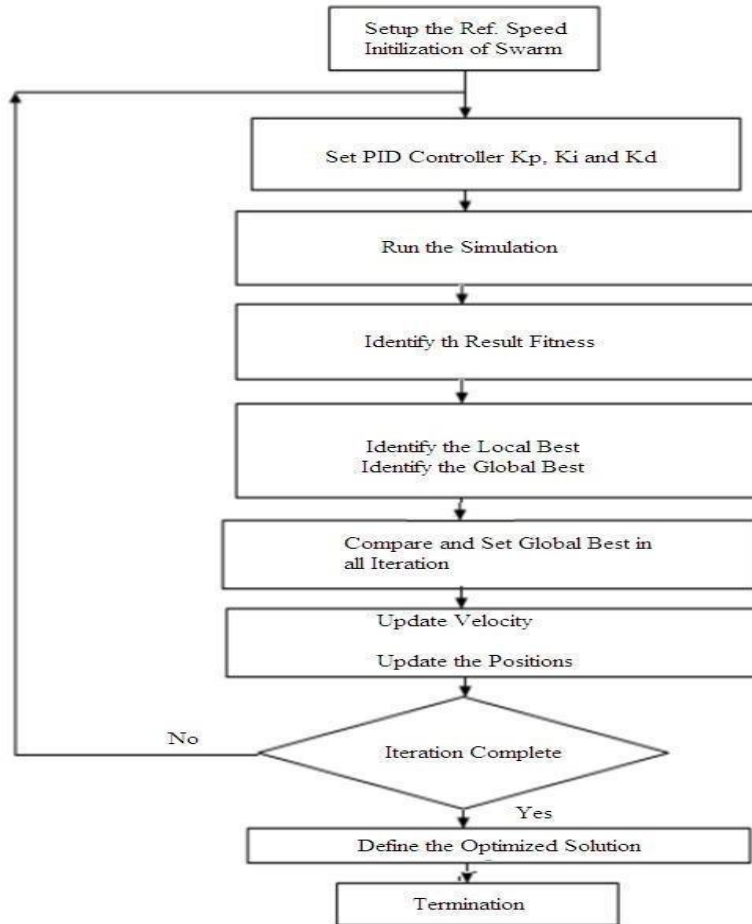
Figure 9: PSO Algorithm for tuning of BLDC Motor Controller
