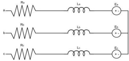
Figure 7: Typical Equivalent Circuit of BLDC Motor
