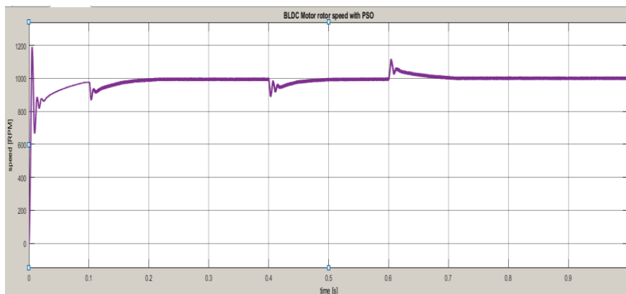
Figure 11: BLDC Motor Rotor Speed with PSO
