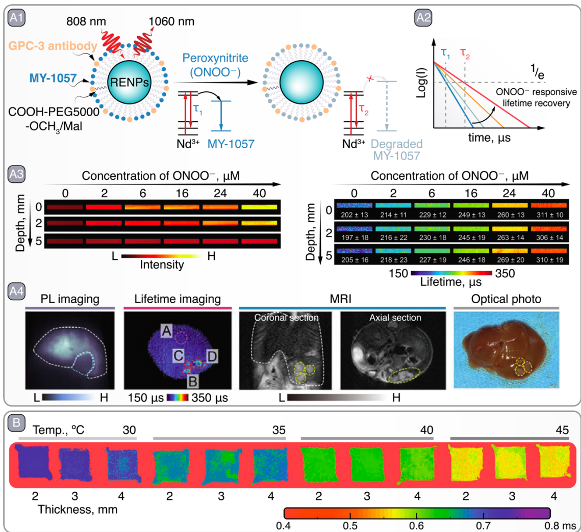
Figure 9. A – Lifetime-based detection of peroxynitrite ( \text{ONOO}^- ) and hepatocellular carcinoma imaging with RENPs: A1 – schematic representation of RENPs engineered for \text{ONOO}^- sensing. A2 – qualitative depiction of \text{Nd}^{3+} ^4F_{3/2} excited state lifetime restoration (measured via 1060 nm emission) due to MY-1057 degradation in the presence of \text{ONOO}^- . A3 – intensity- (left) and lifetime-based (right) imaging of RENPs containing capillaries as a function of \text{ONOO}^- concentration and imaging depth. A4 – PL intensity- and lifetime-based imaging, as well as MRI, of a mouse bearing multiple HCC lesions, and optical photo of the dissected liver. Images reproduced and adapted with permission from reference 90. B – lifetime-based PL thermometry with RENPs at various imaging depths and temperatures. Images reproduced and adapted with permission from reference 94.
