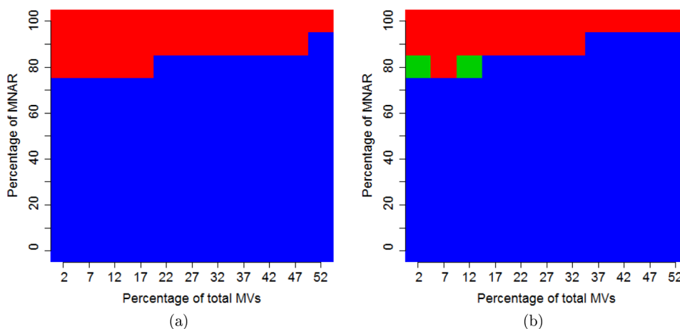
Figure 4. (a) Comparison of SVDimpute and MinDet on the simulated data set. (b) Comparison of MLE and MinDet on the real data set. Red color indicates an outperformance of MinDet, a blue color, an underperformance of MinDet, and a green color, a difference of performance that is not significant with a p -value threshold of 5%.
