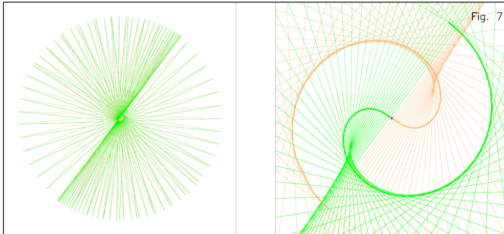
Fig. 6 uses the last hundred vectors ( n=3083\div 3183 ) that converge on (Of), Fig. 7 uses the first hundred vectors ( n=3183\div 3283 ) that diverge from (Of); I added a small circle to indicate the origin and two spirals connecting the midpoints of the vectors.
