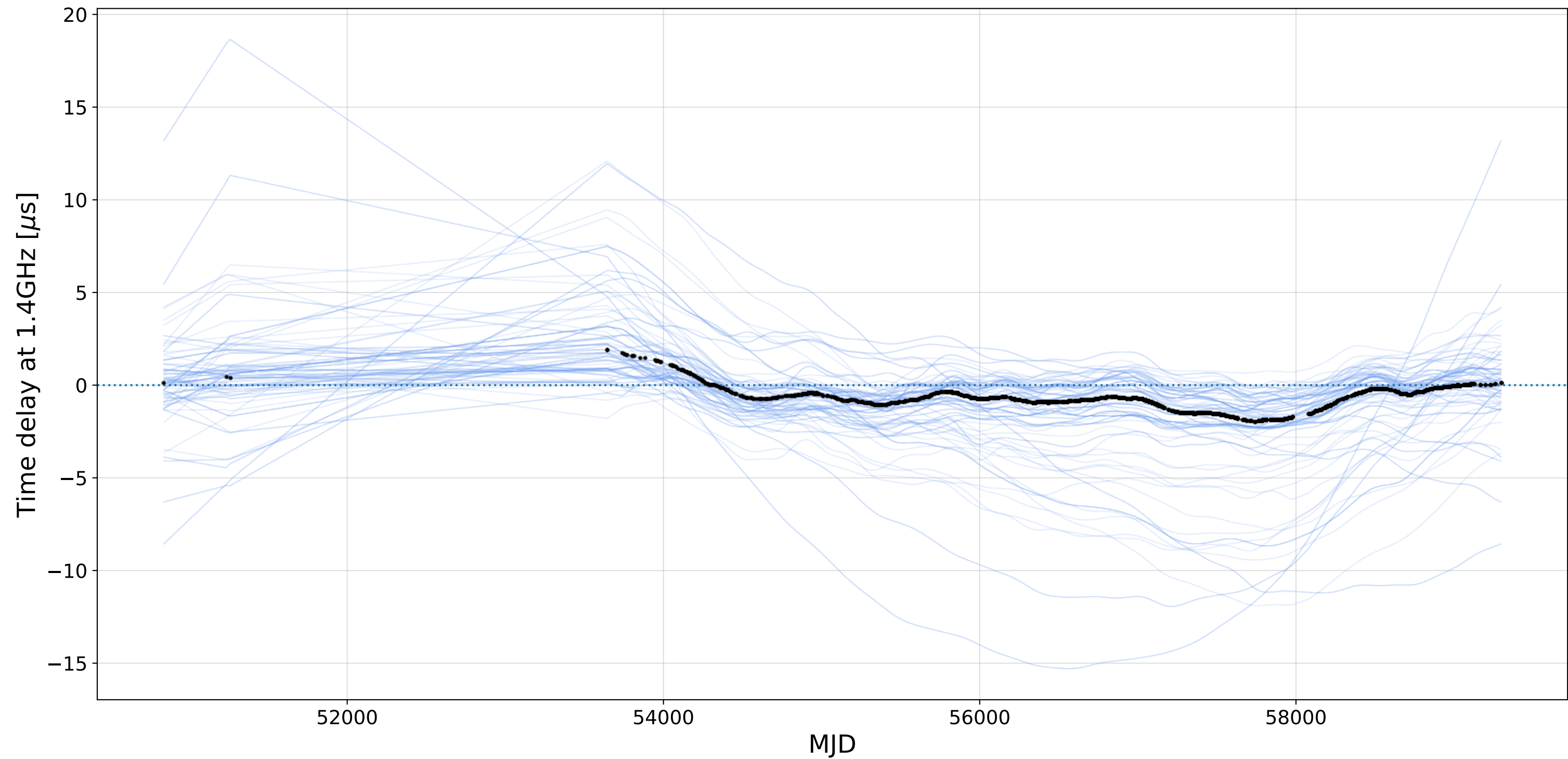
J1024-0719 - EPTA DR2full+, DM variations reconstructions
