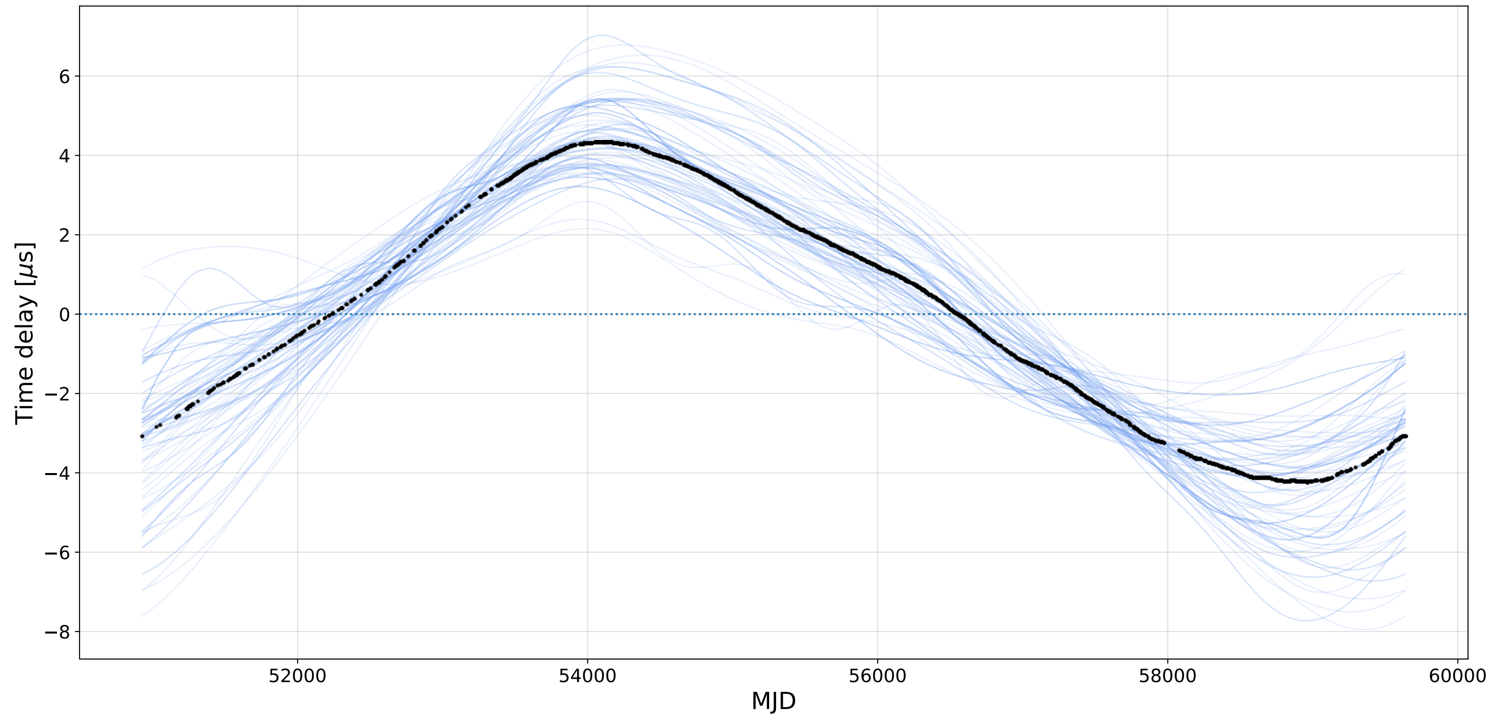
J0613-0200 - EPTA DR2full+, Red noise reconstructions
