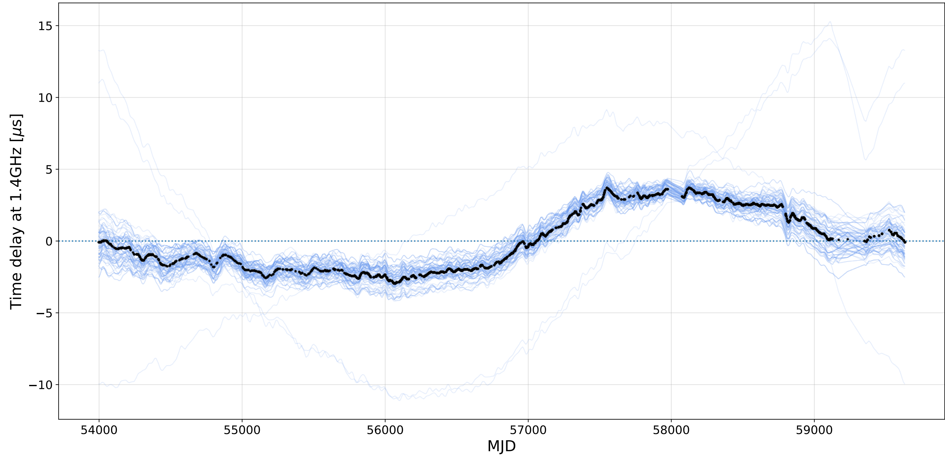
J1600-3053 - EPTA DR2full+, DM variations reconstructions
