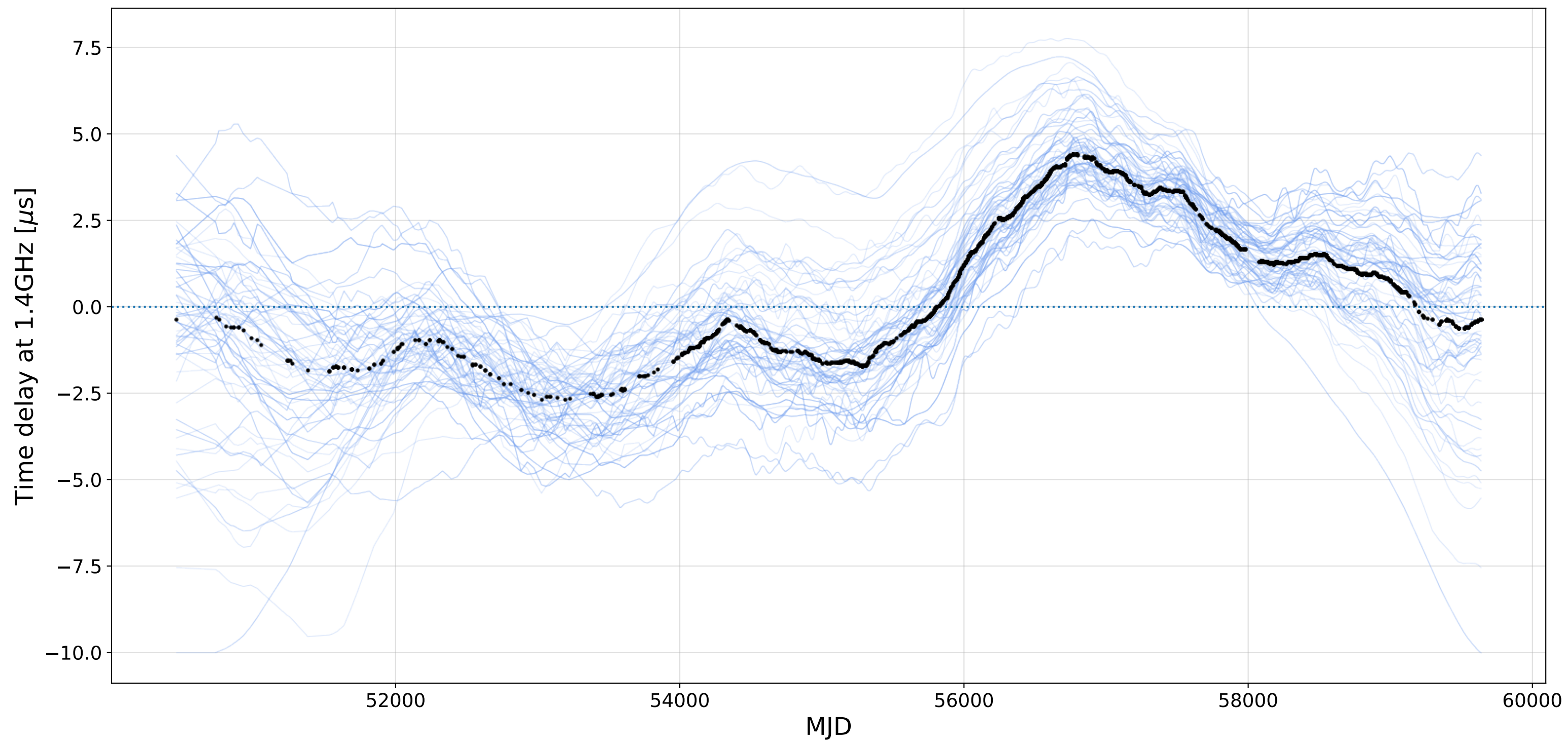
J0751+1807 - EPTA DR2full+, DM variations reconstructions
