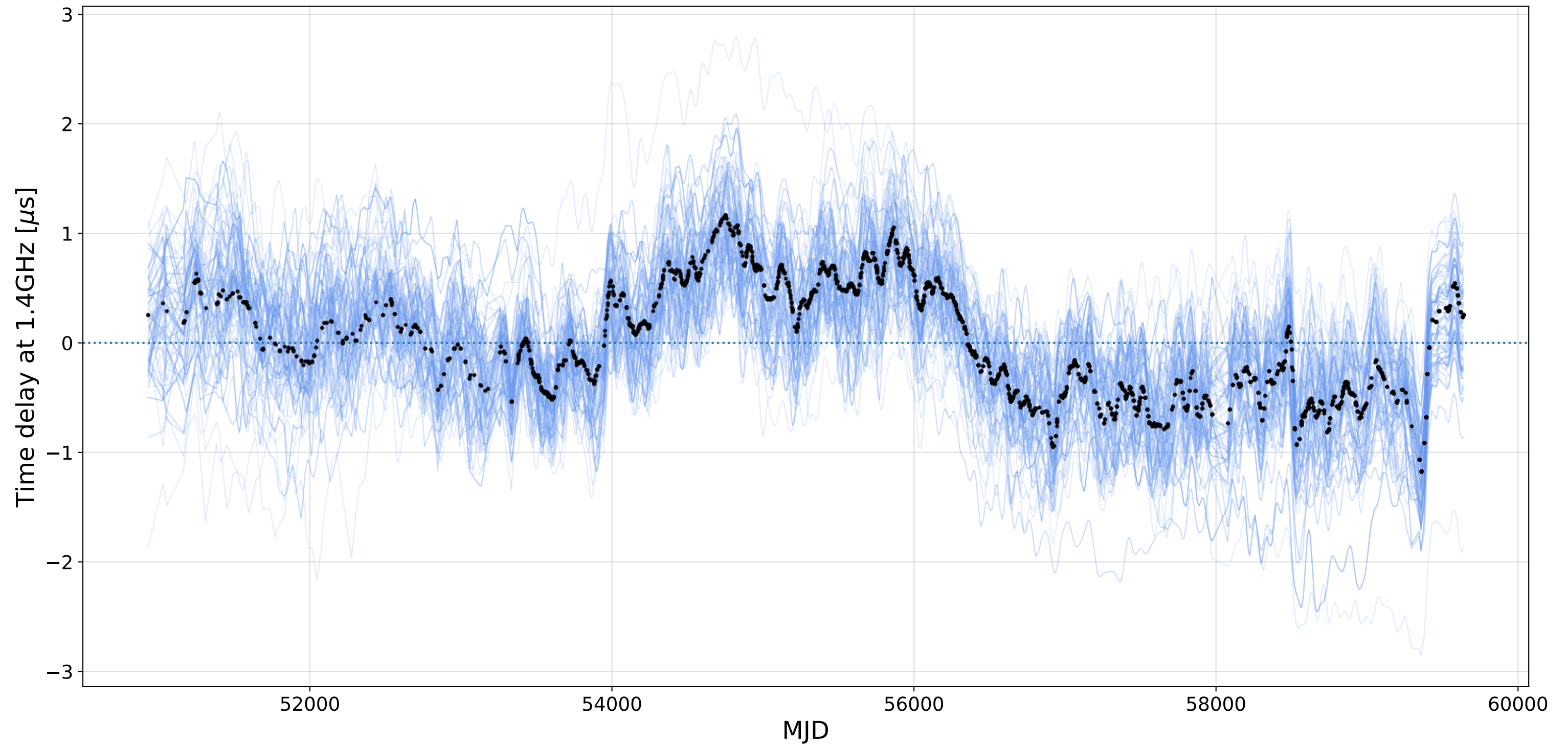
J0613-0200 - EPTA DR2full+, DM variations reconstructions
