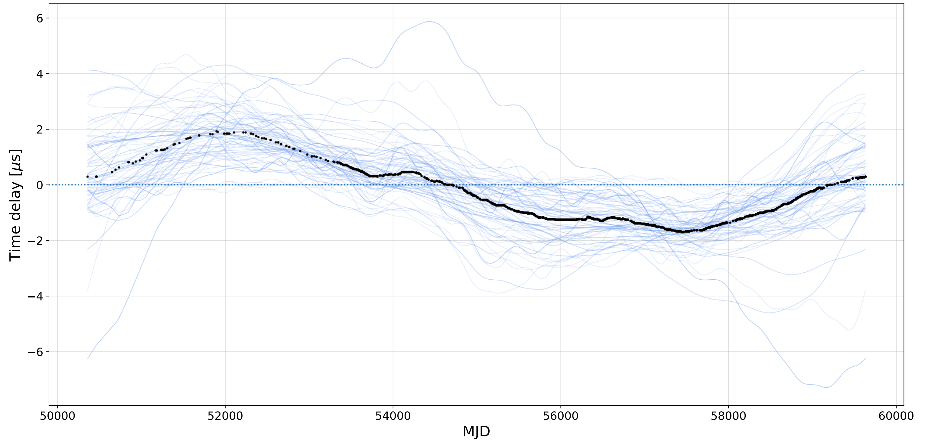
J1022+1001 - EPTA DR2full+, Red noise reconstructions
