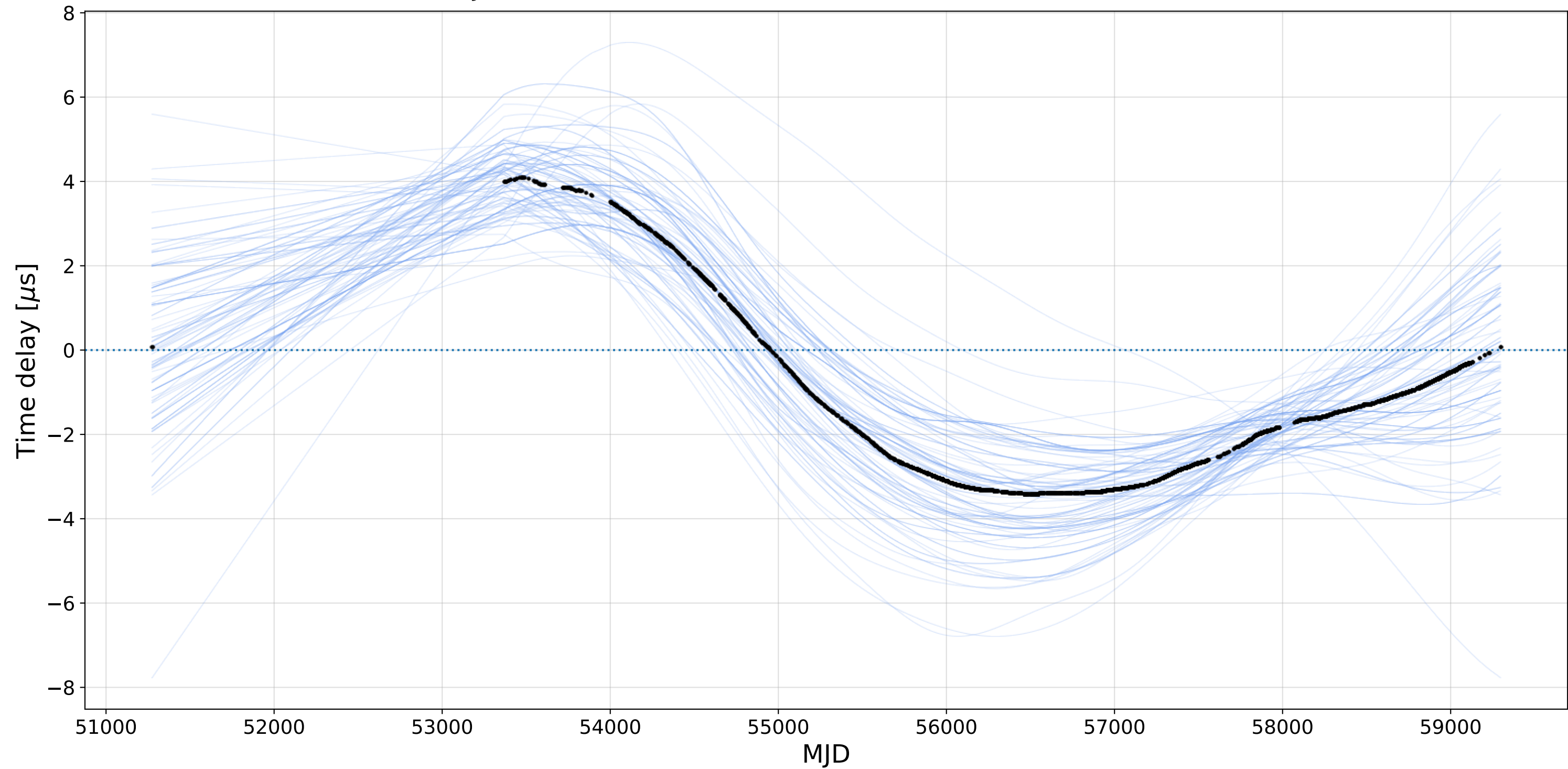
J0030+0451 - EPTA DR2full+, Red noise reconstructions
