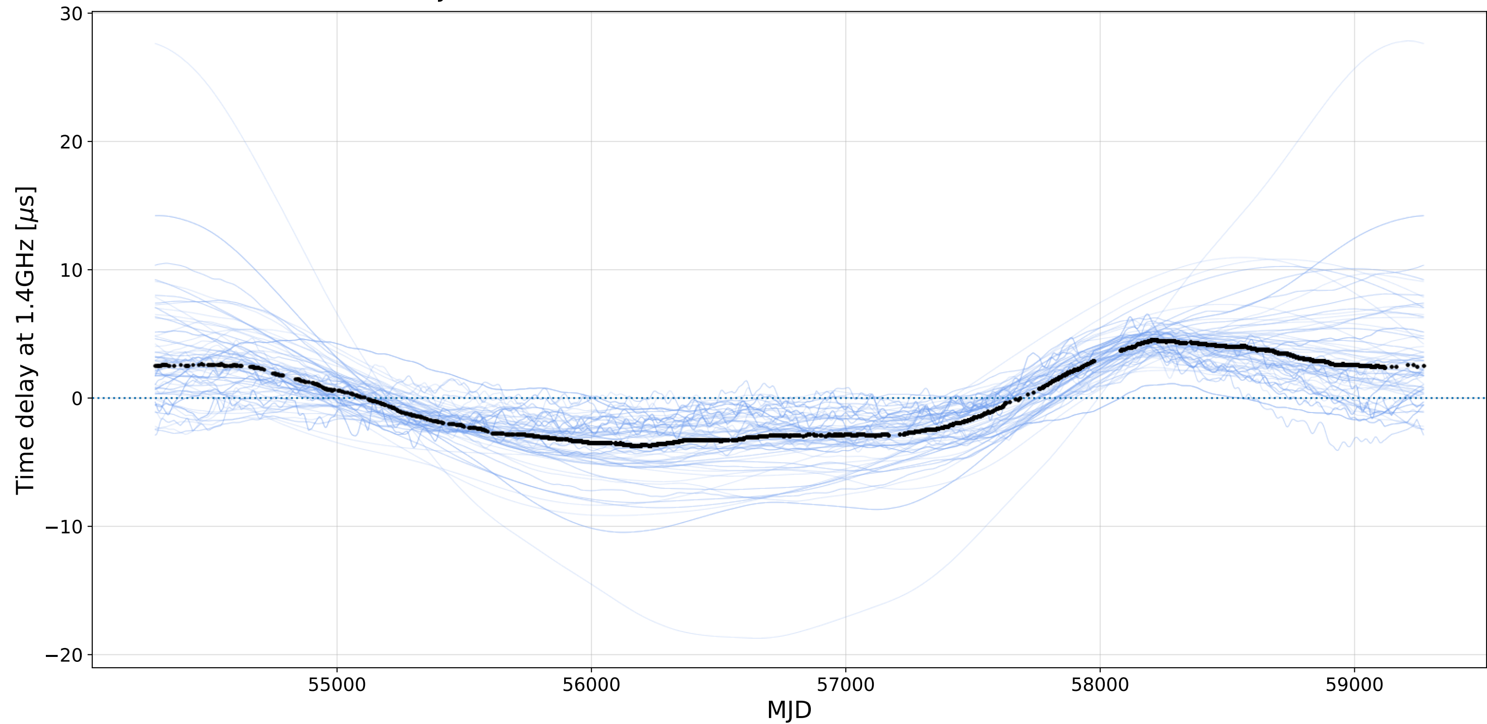
J0900-3144 - EPTA DR2full+, DM variations reconstructions
