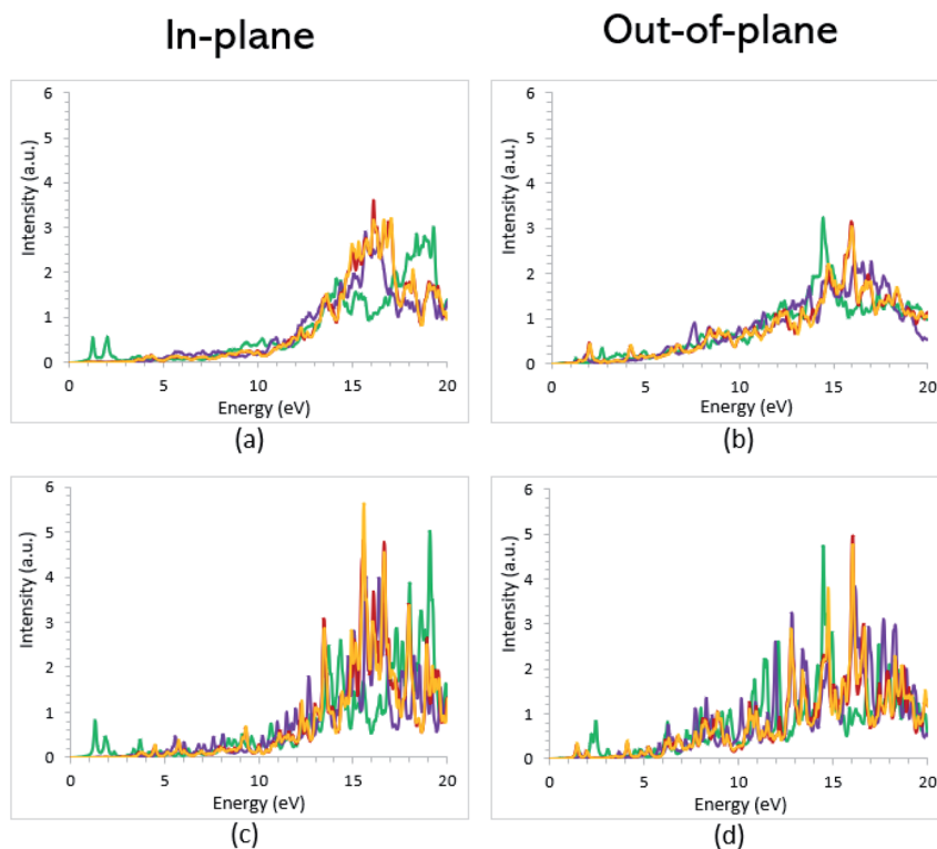
Fig. 6 Energy loss function spectra of VO 2 (B) PP (green), VO 2 (B) LP (purple), VO 2 (B) PPD (red), and VO 2 (B) LPD (orange) structures along the in-plane and out-of-plane polarizations, as predicted by RPA + PBE (a and b) and RPA + PBE + U (c and d).
