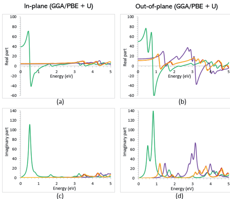
Fig. 5 Imaginary and real parts of the dielectric function of VO 2 (B) PP (green), VO 2 (B) LP (purple), VO 2 (B) PPD (red), and VO 2 (B) LPD (orange) structures along the in-plane (a and c) and out-of-plane (b and d) polarizations, as predicted by RPA + PBE + U.
