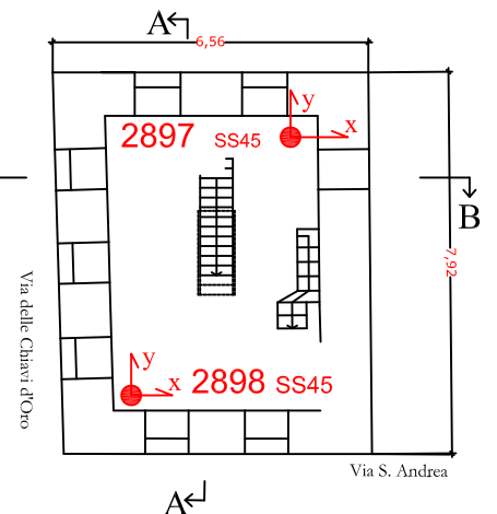
Level 5 (+39.88)
