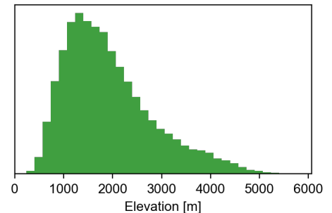
Figure 3.2. Distribution of elevation within in the mountain range [11].
