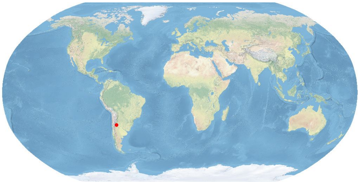
Location of the Sierras Pampeanas mountain range [1][2].
