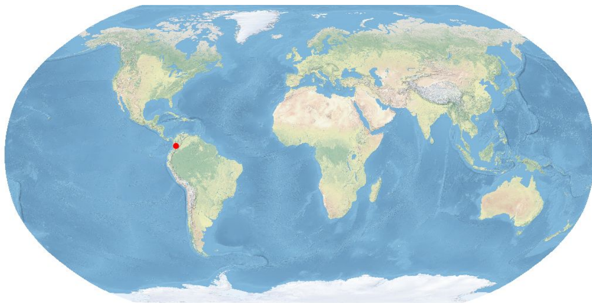
Location of the Cordillera Central (Northern Andes) mountain range [1][2].
