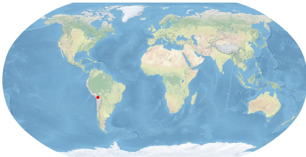
Location of the Altiplano mountain range [1][2].
