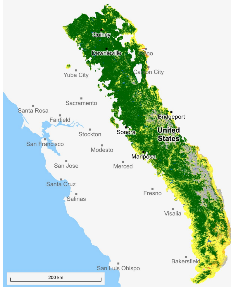
Figure 2.1. Land Cover
