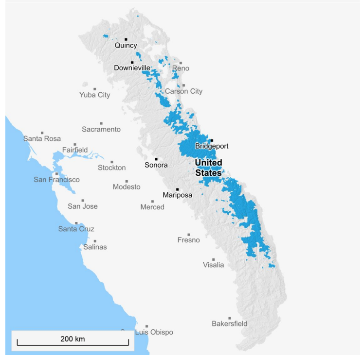
Figure 6.4. Mean Snow Covered Area (February)
