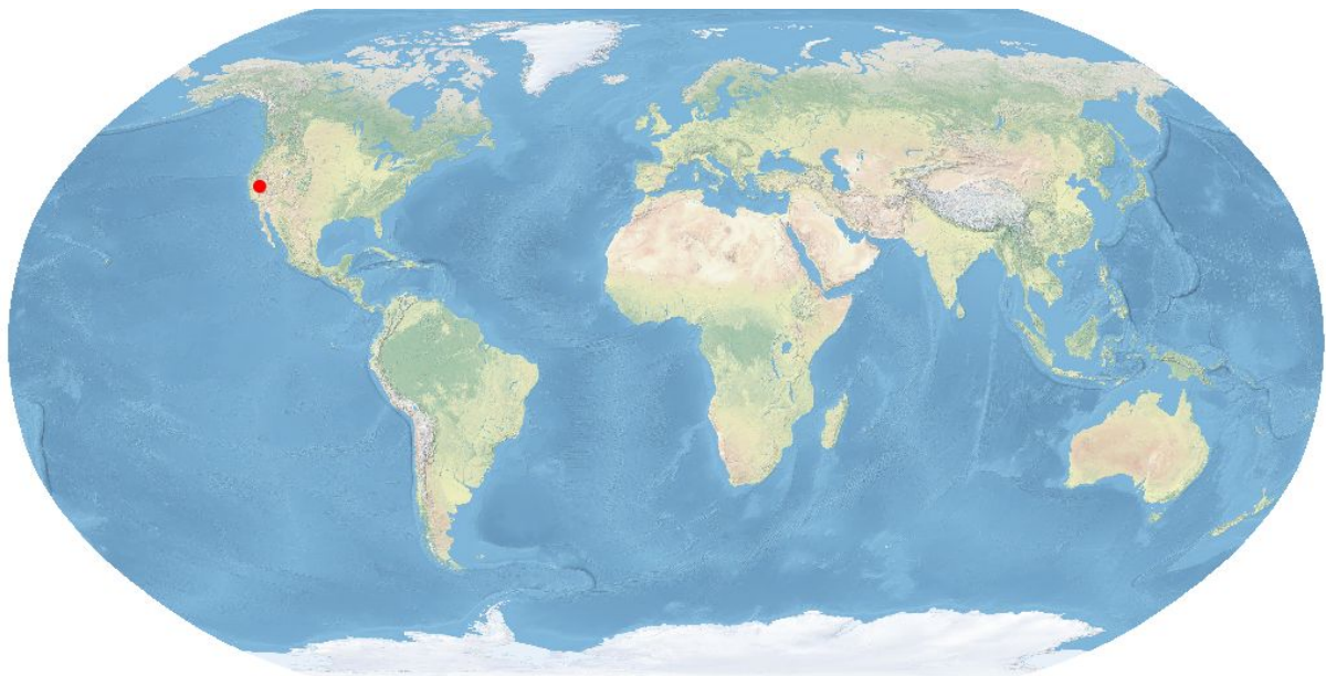
Location of the Sierra Nevada (USA) mountain range [1][2].
