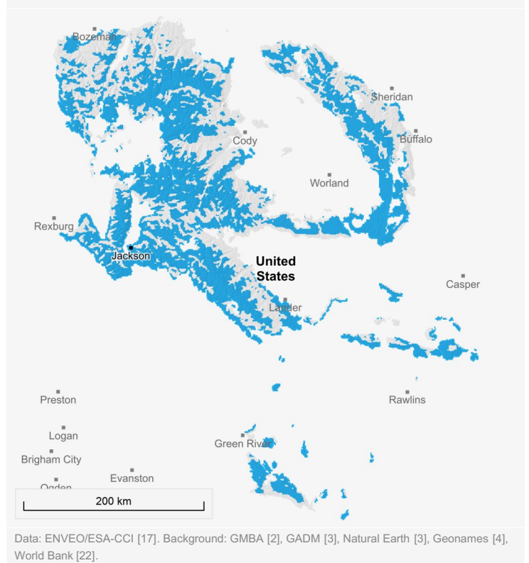
Figure 6.4. Mean Snow Covered Area (February)
