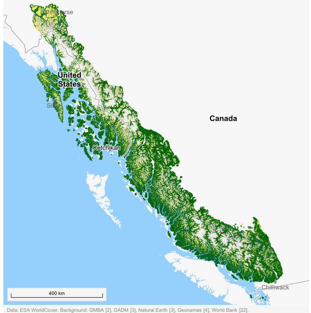
Figure 2.1. Land Cover
