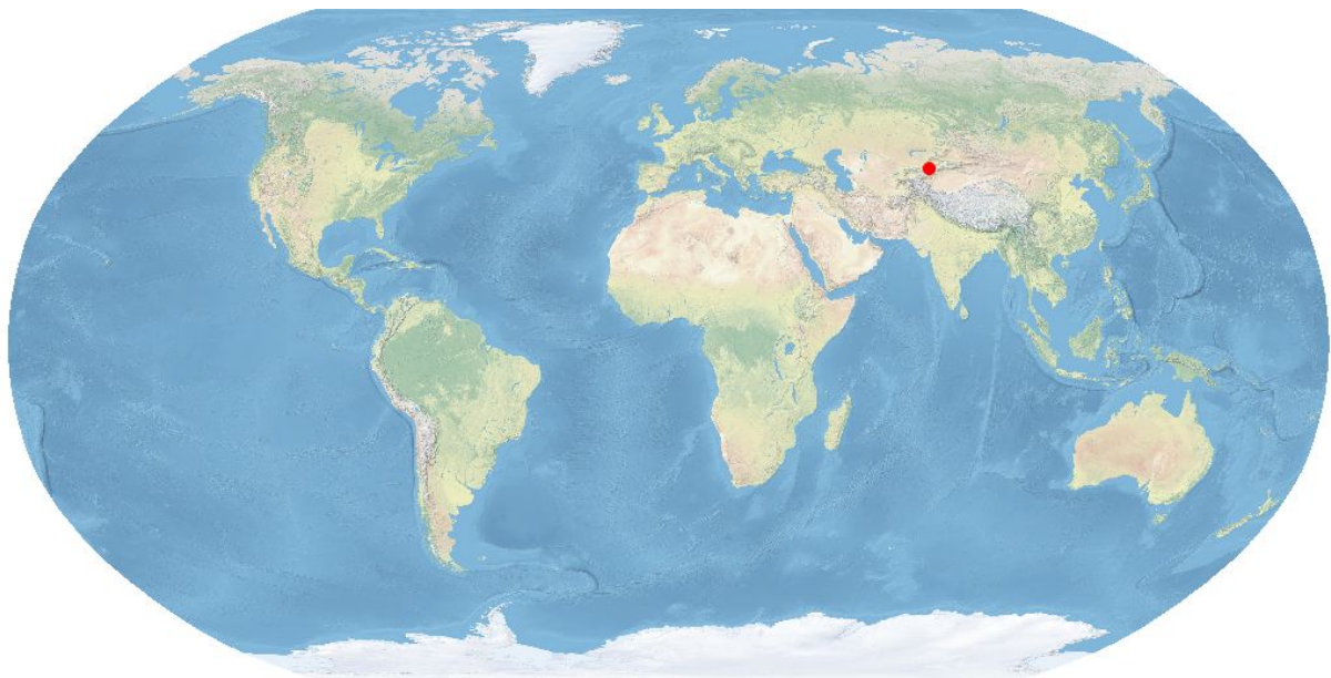
Location of the Tian Shan mountain range [1][2].
