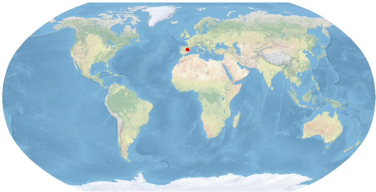
Location of the Sistema Iberico mountain range [1][2].
