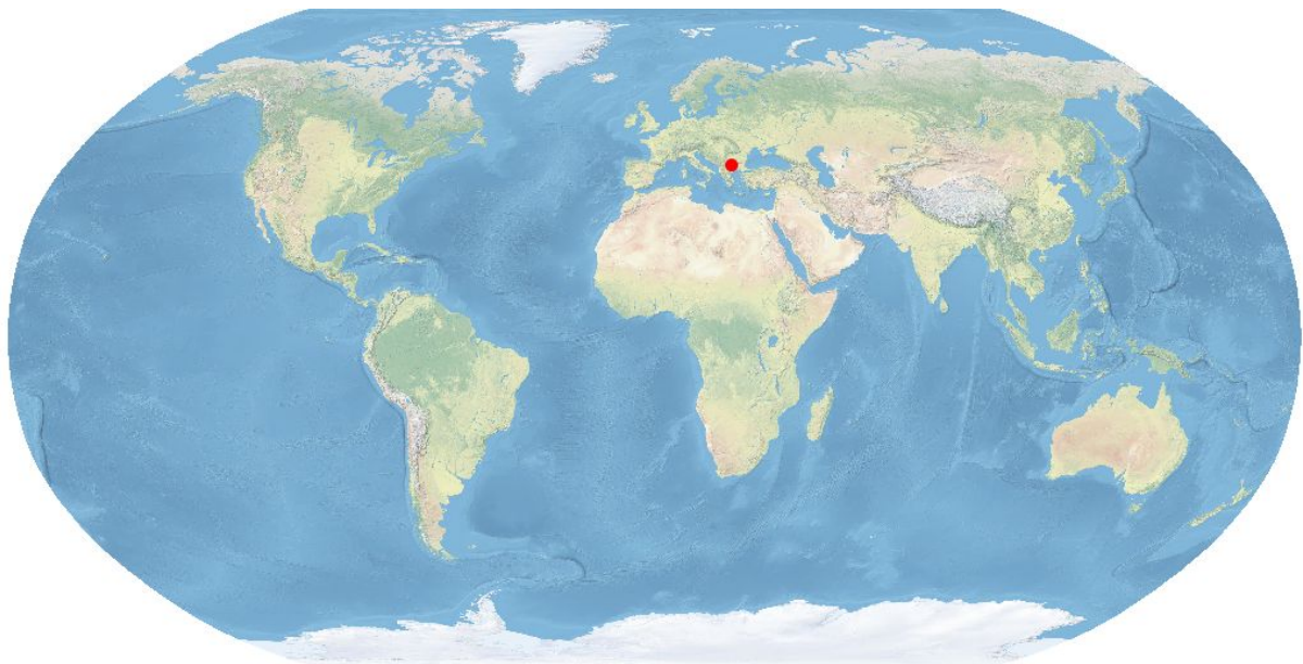
Location of the Rila-Rhodope Massif mountain range [1][2].
